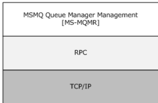
Figure 1: Protocol relationships
