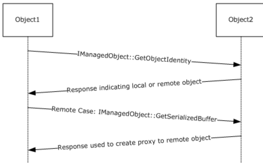
Figure 3: IManagedObject request-response
