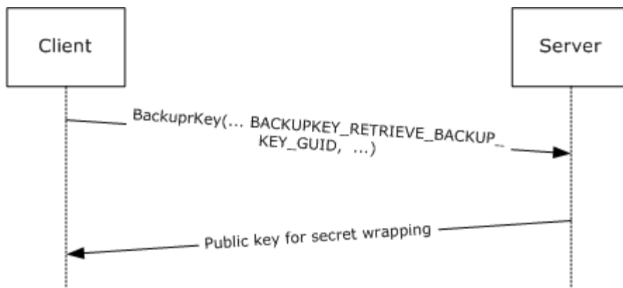
Figure 3: Retrieving the server's public key for client-side secret wrapping
