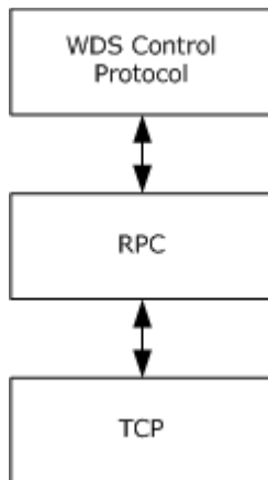
Figure 1: Protocol relationships
