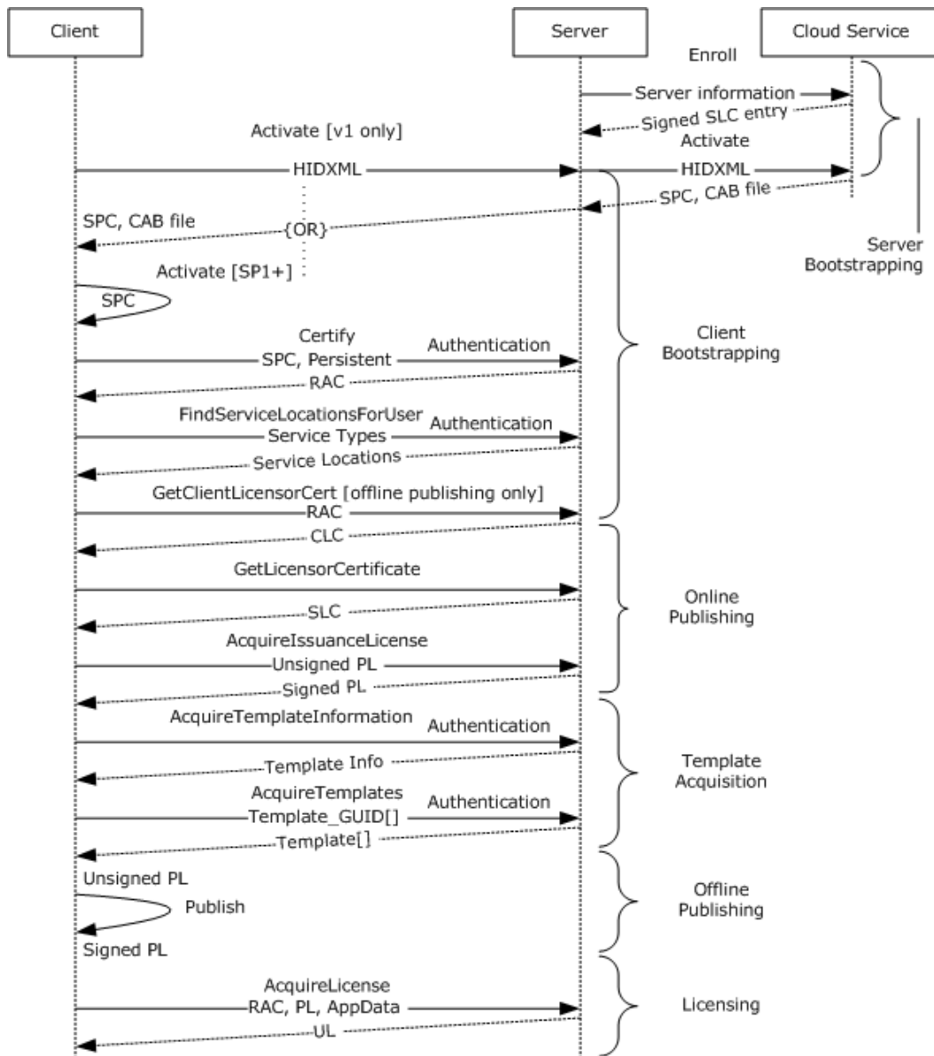
Figure 5: Protocol operation
