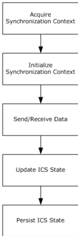
Figure 1: Synchronization states
