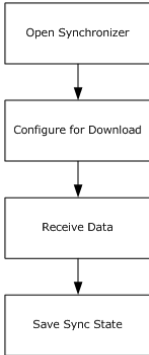
Figure 2: Download details
