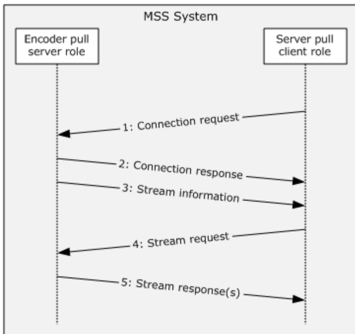
Figure 16: Media server pull from encoder communication flow
