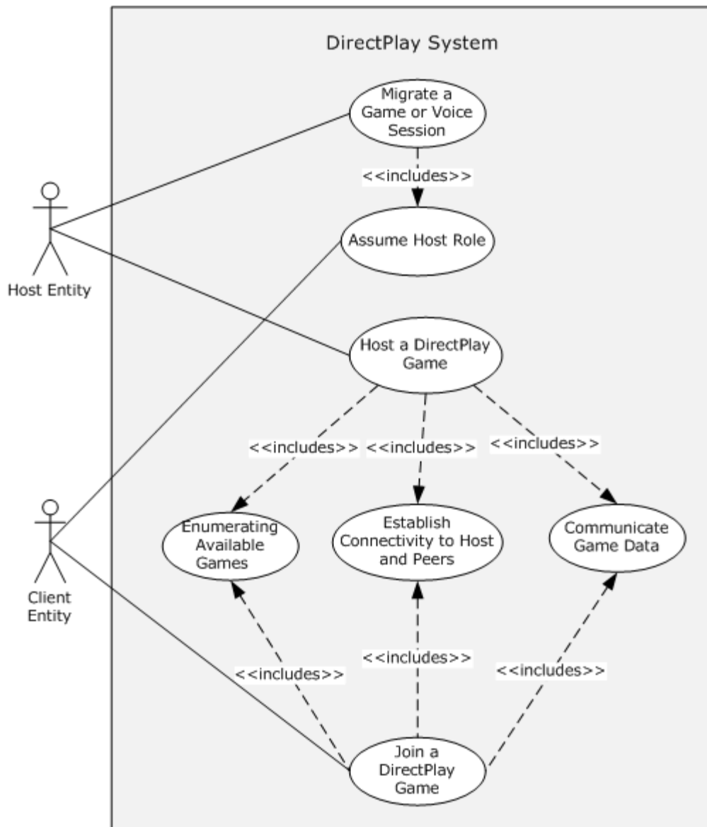
Figure 3: DirectPlay System use cases
