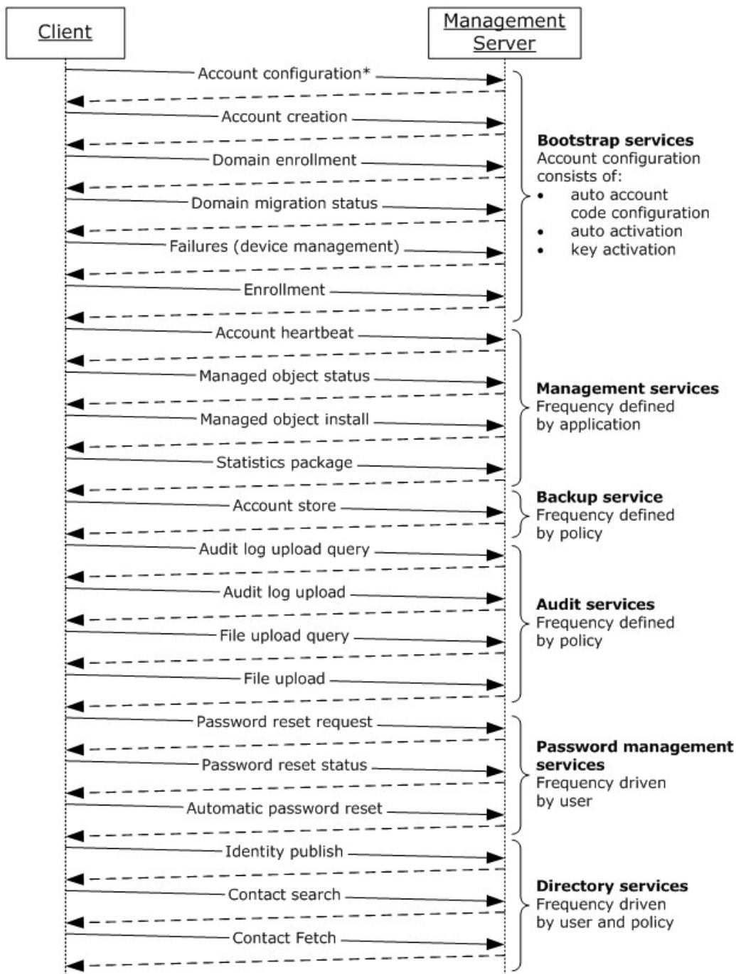
Figure 4: Message sequence between protocol client and protocol server
