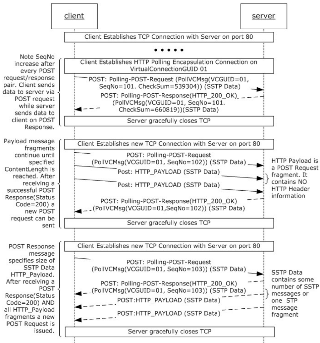
Figure 27: Polling connection data exchange
