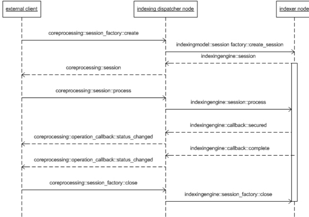
Figure 3: Sessions and callback messages
