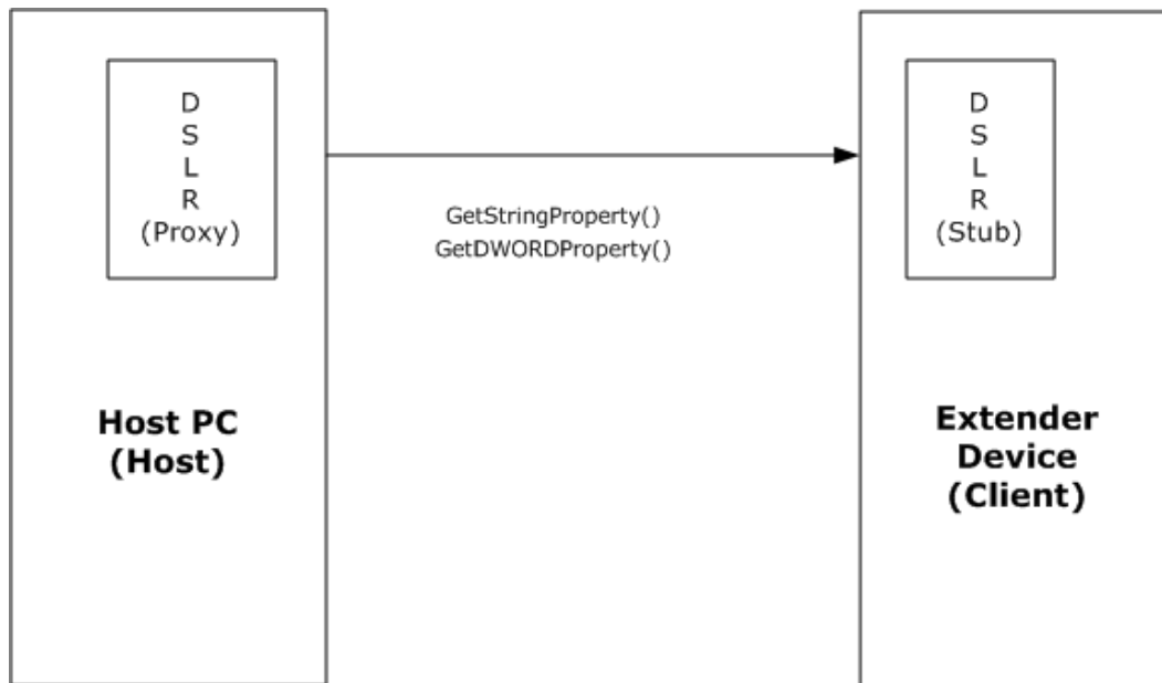
Figure 1: Device Session Property Access Protocol block diagram
