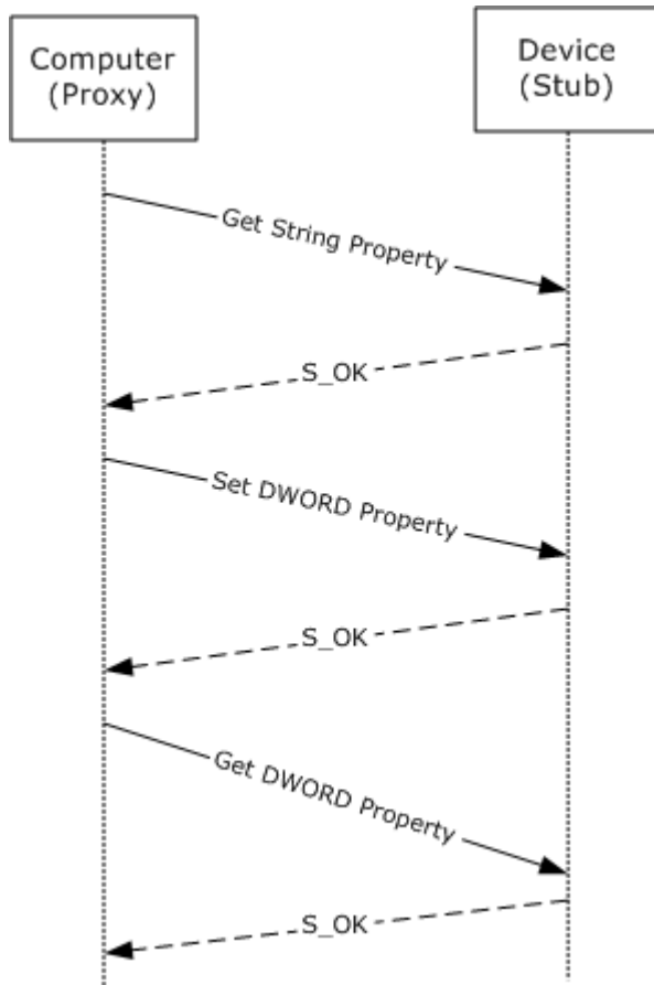
Figure 3: DSPA Protocol sequence diagram
