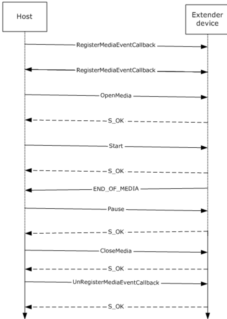
Figure 5: Sequence diagram for MS-DMCT
