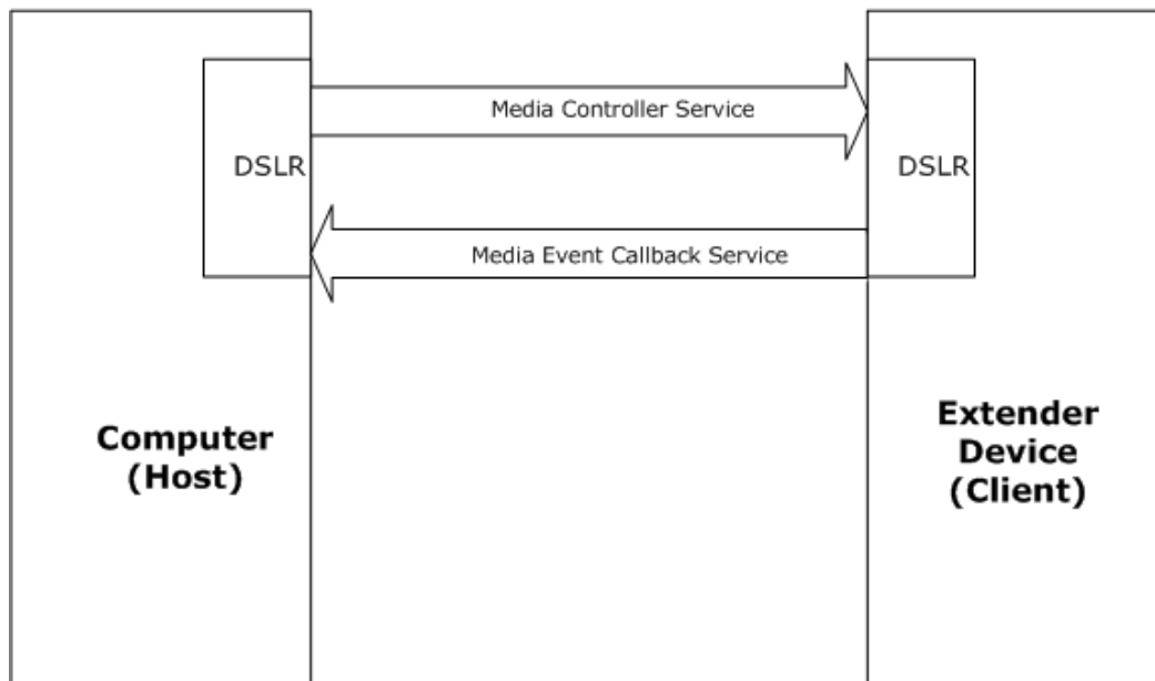
Figure 1: MS-DMCT protocol block diagram
