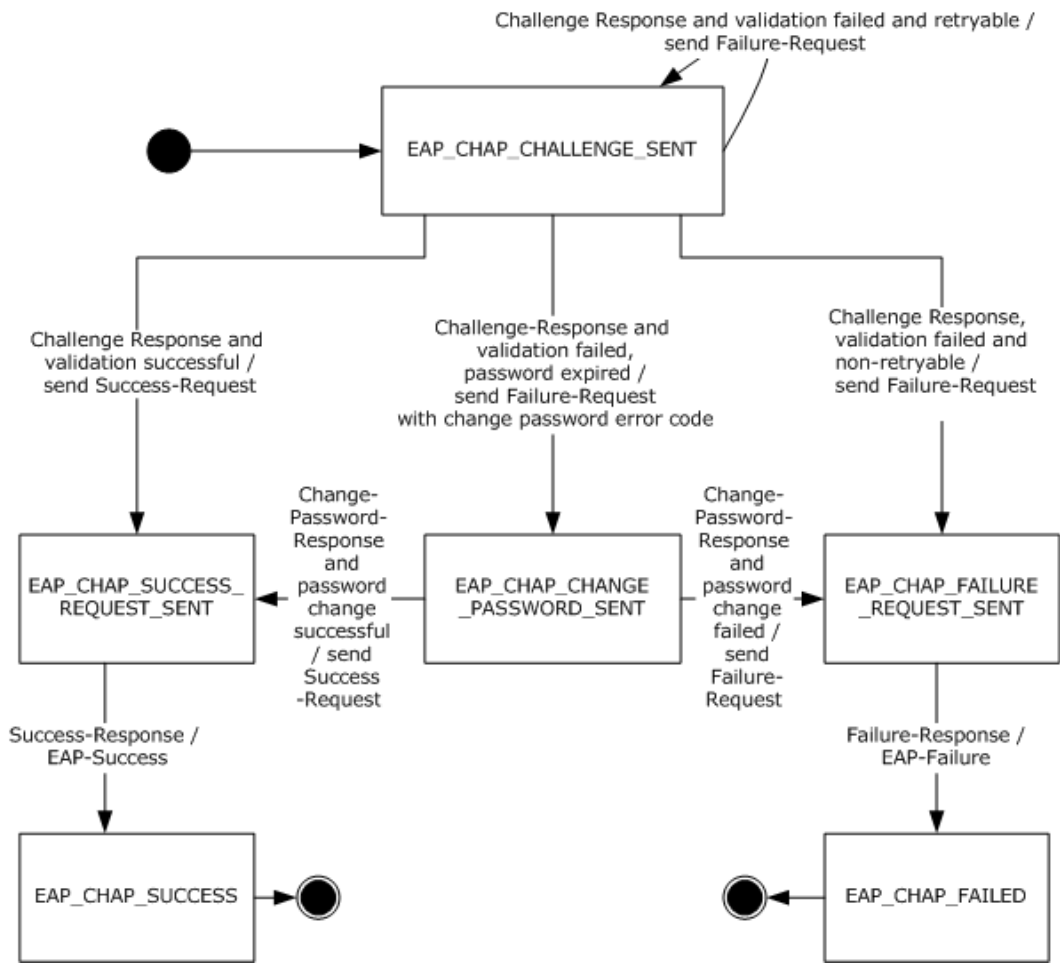
Figure 4: EAP-CHAP server state machine
