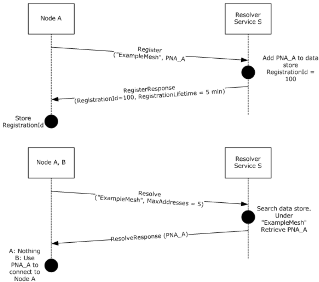
Figure 1: Register and resolve sequences
