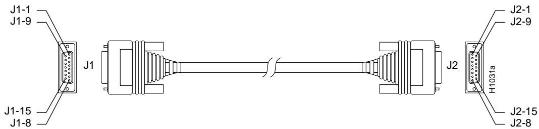
Figure 2 Ethernet (AUI) Cable Assembly
