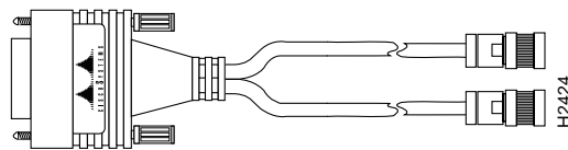
Figure 8 E1 Interface Cable for 120-Ohm, Balanced Connections with Twinax Connectors
