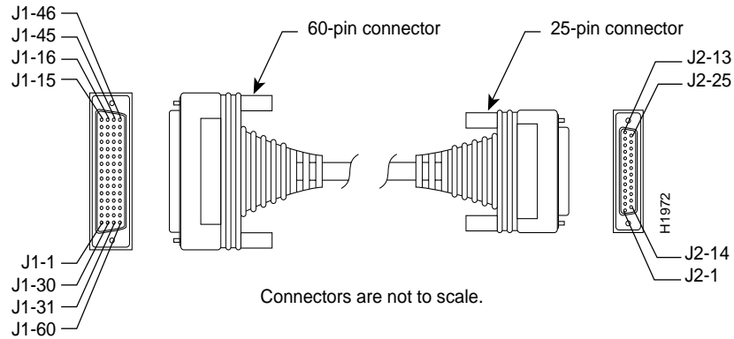
Figure 19 EIA-530 Serial Cable Assembly
