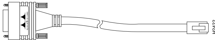
Figure 9 E1 Interface Cable for 120-Ohm, Balanced Connections with an RJ-45 Connector
