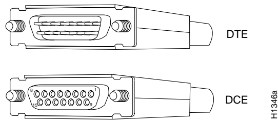
Figure 16 X.21 Adapter Cable Connectors, Network End
