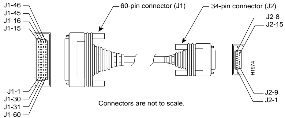
Figure 17 X.21 Serial Cable Assembly
