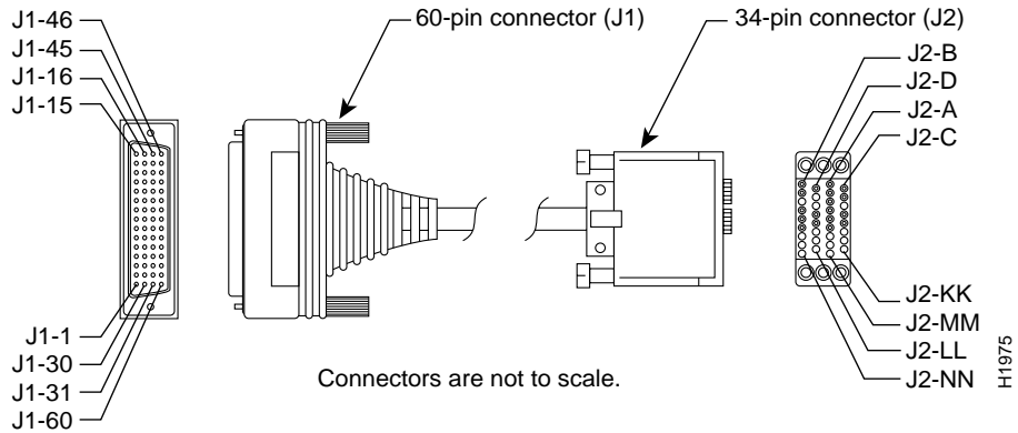
Figure 15 V.35 Serial Cable Assembly
