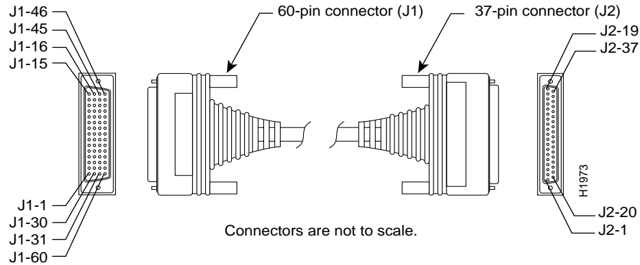
Figure 13 EIA/TIA-449 Serial Cable Assembly
