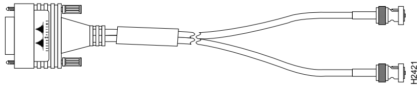
Figure 6 E1 Interface Cable for 75-Ohm, Unbalanced Connections with BNC Connectors
