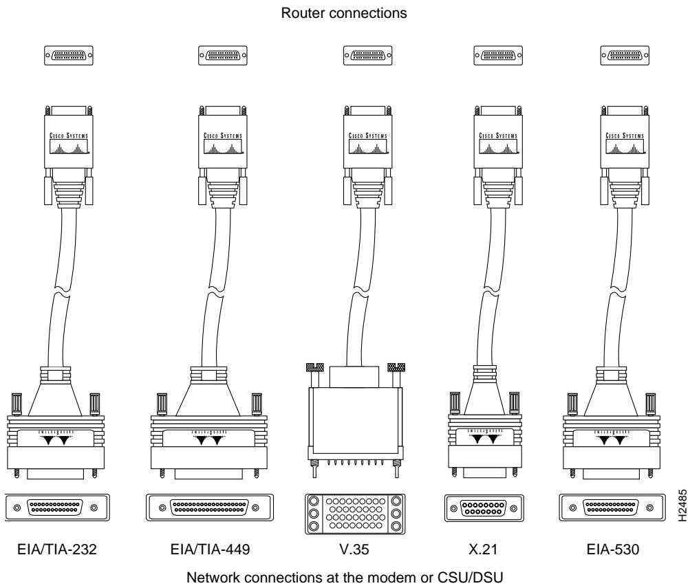
Figure 20 Smart Serial Interface Adapter Cables
