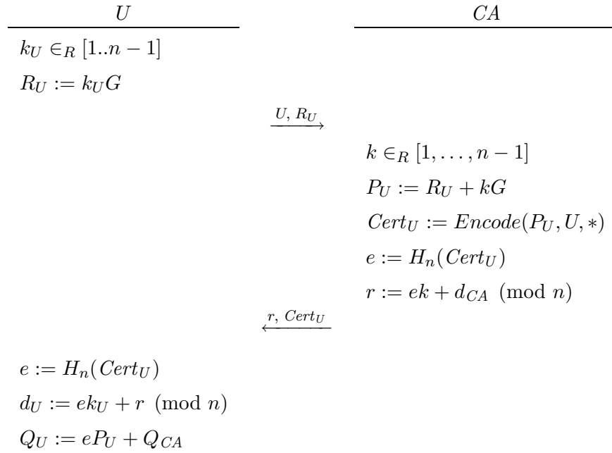
Figure 1: The ECQV certificate issuance protocol.
