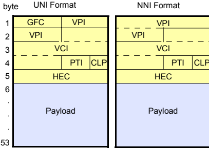
Figure 1 ATM Cell format
