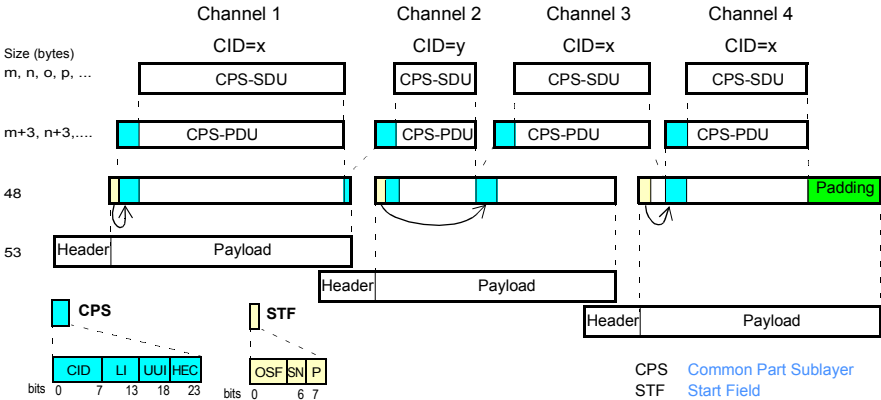
Figure 11 AAL2 format
