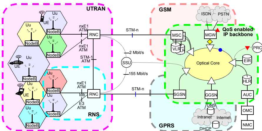
Figure 23 UMTS/3G architecture
