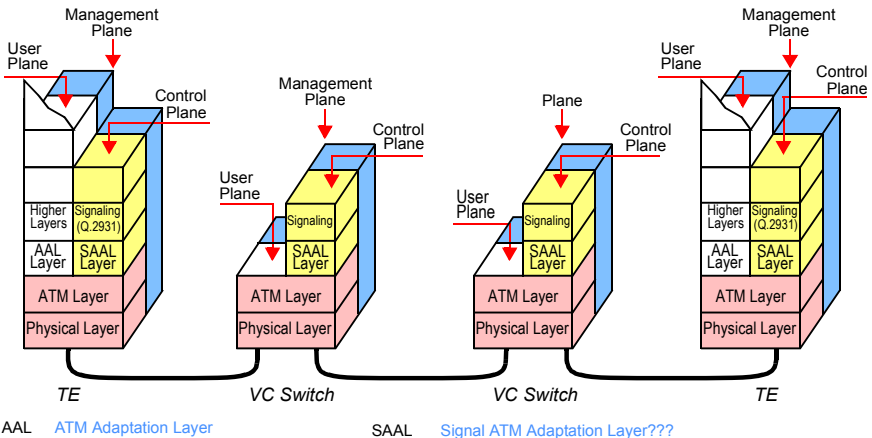
Figure 6 Layers and planes implemented in terminal equipment (TE) and switches
