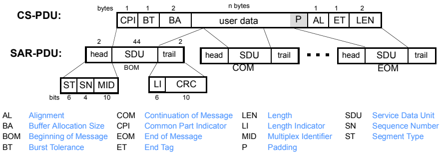
Figure 12 AAL3/4 format
