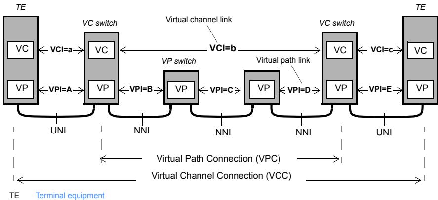
Figure 5 Virtual channel connection and virtual path connection
