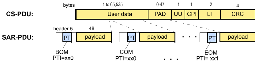
Figure 13 AAL5 format
