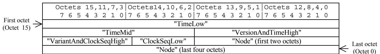
Figure 1 – Position of UUID fields in the binary representation
