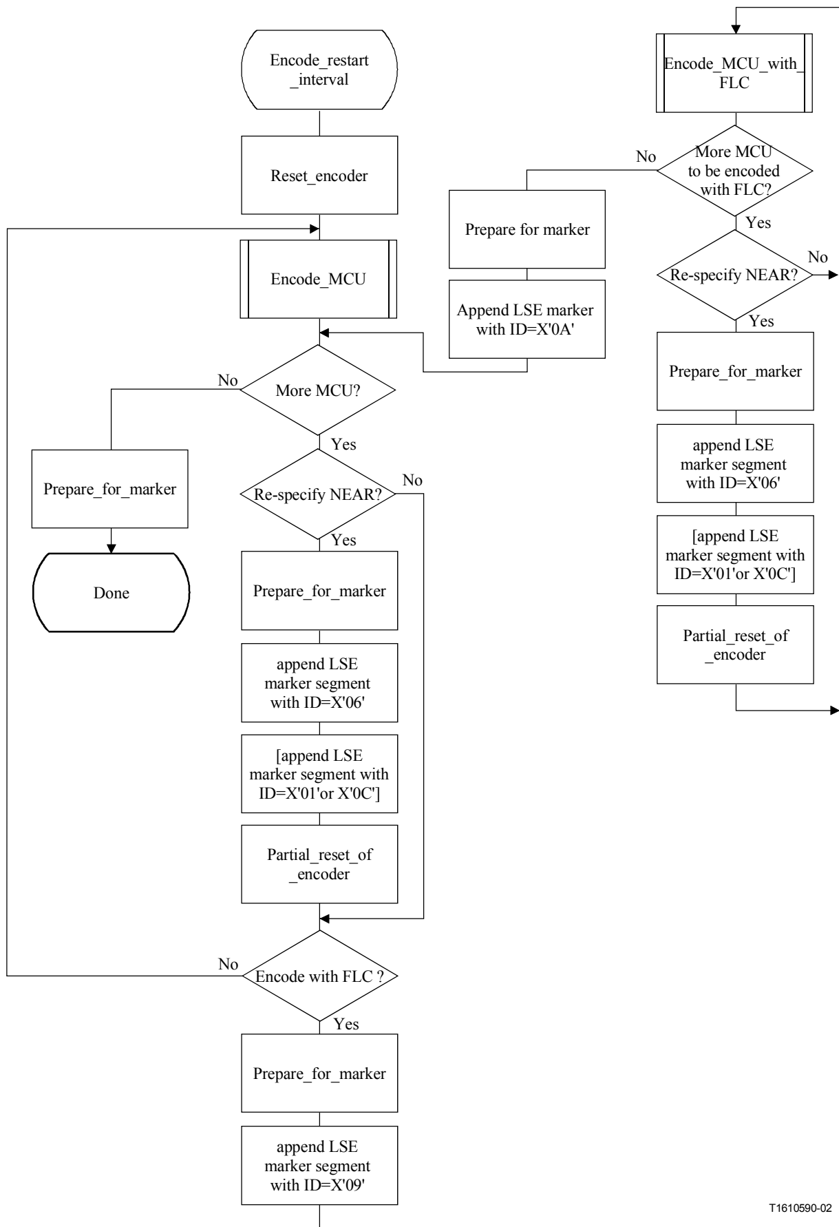
Figure H.1 – Control procedure for encoding a restart interval
