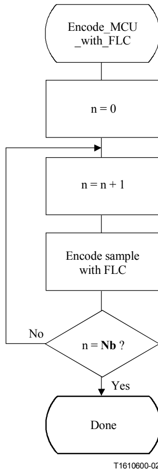
Figure H.2 – Control procedure for encoding a minimum coded unit (MCU) with fixed length coding (FLC)
