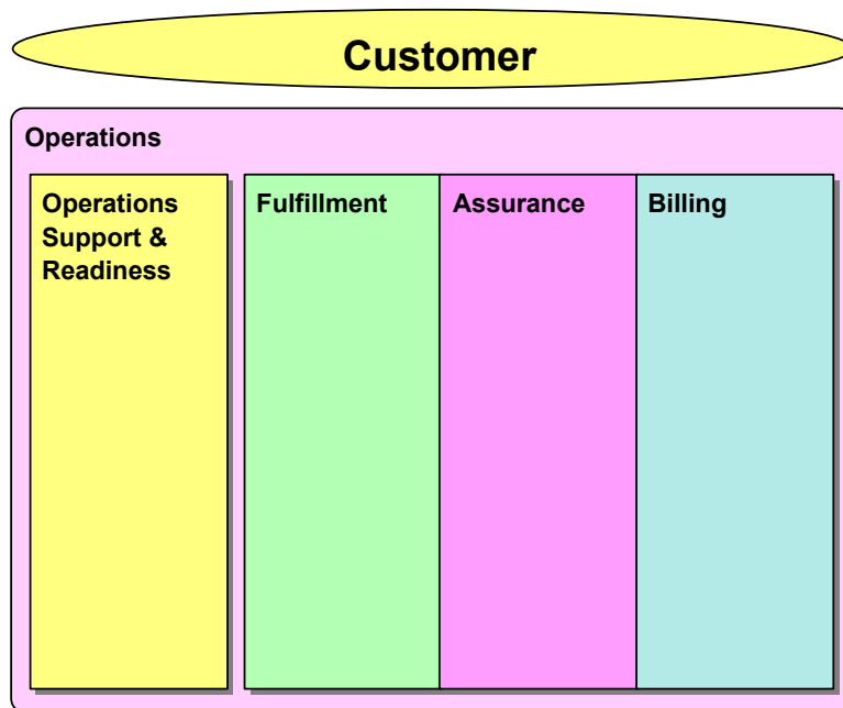
Figure 5 - eTOM OPS Vertical Process Groupings
