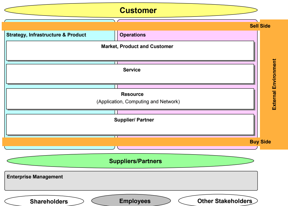
Figure 10 - the eTOM framework and the external environment
