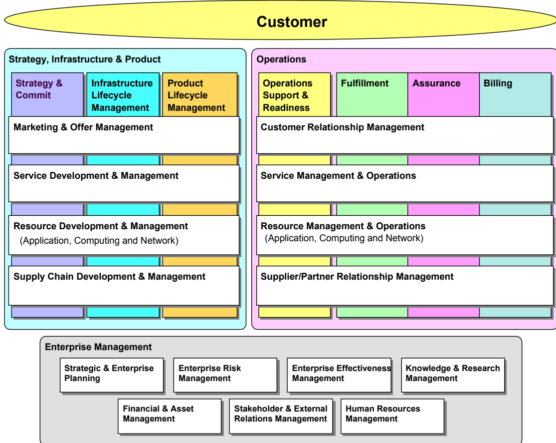
Figure 4 - eTOM Level 0 View of Level 1 Process Groupings
