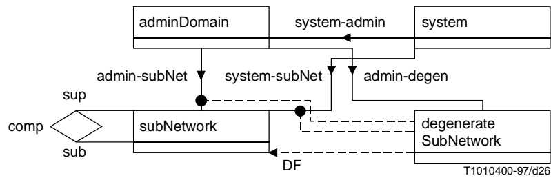
Figure I.1/Z.360 – Example GDMO specification
