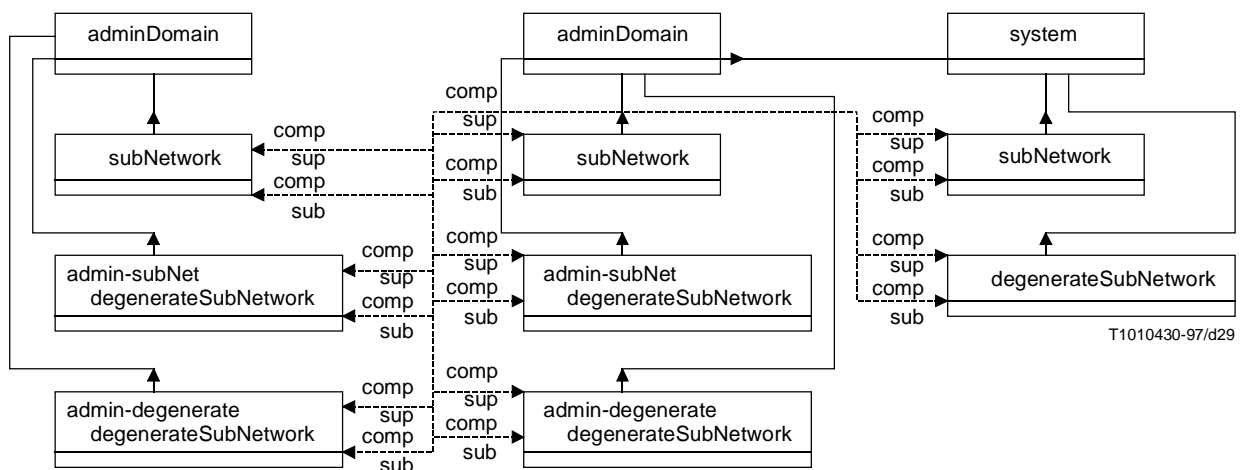
Figure I.4/Z.360 – Example classes prepared for possible instantiation
