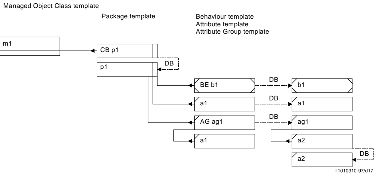
Figure 17/Z.360 – Depiction of some detailed references from an alphanumeric specification
