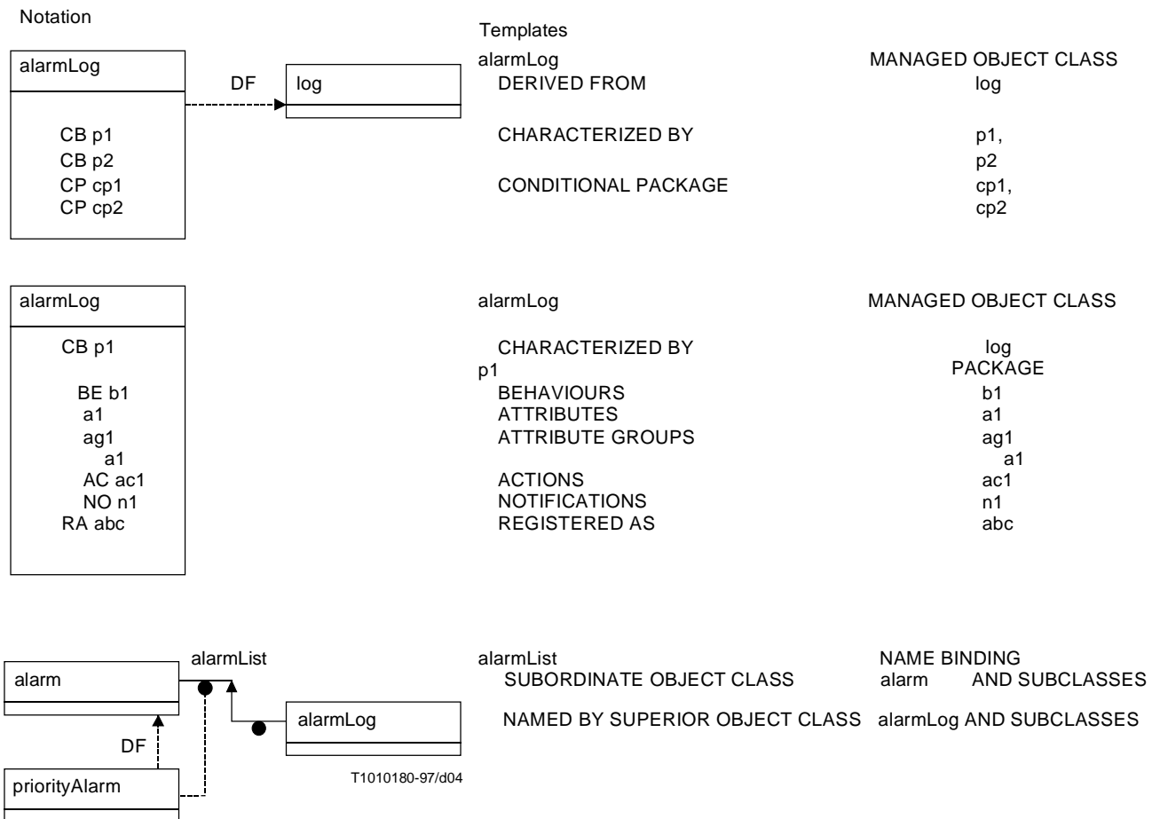
Figure 4/Z.360 – Examples of shorthand and combined notations
