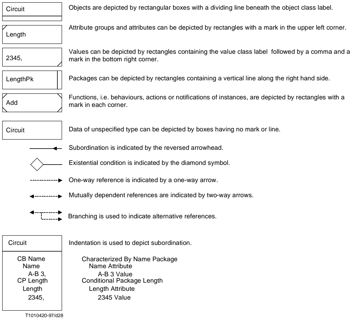
Figure I.3/Z.360 – Graphic instantiation language
