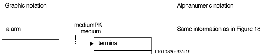
Figure 19/Z.360 – Abbreviated notation
