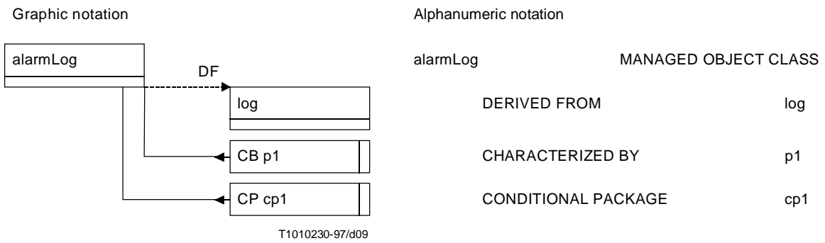
Figure 9/Z.360 – Abbreviated notation
