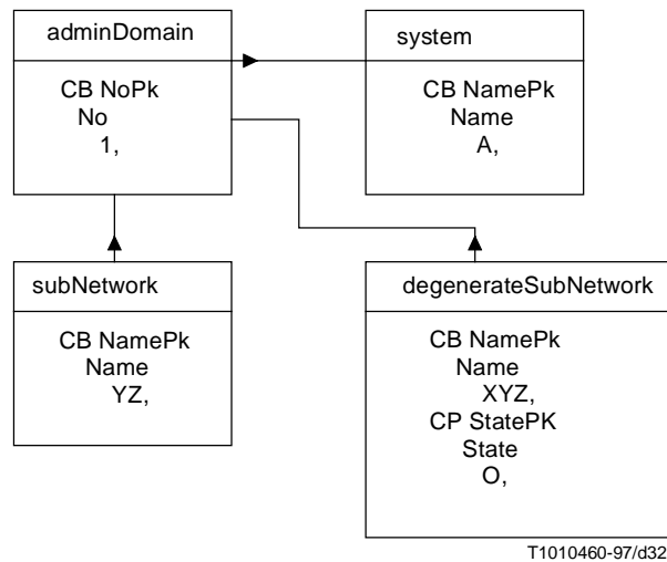
Figure I.7/Z.360 – Example instances with attributes
