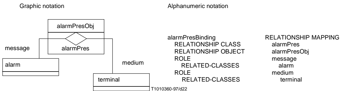
Figure 22/Z.360 – Relationship Mapping template
