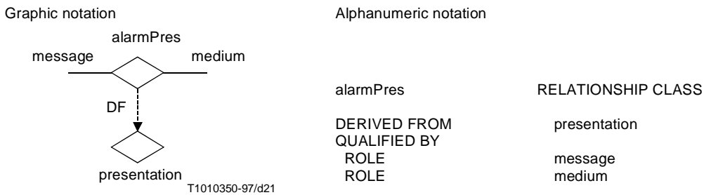
Figure 21/Z.360 – Relationship Class template
