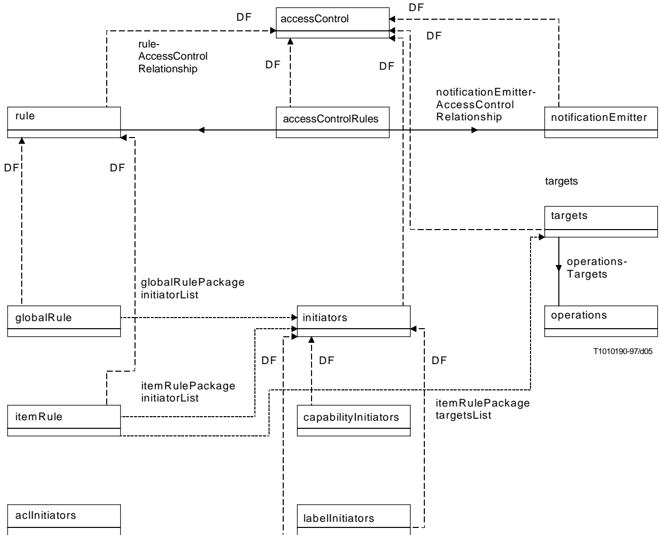
Figure 5/Z.360 – Example compact graphic notation
