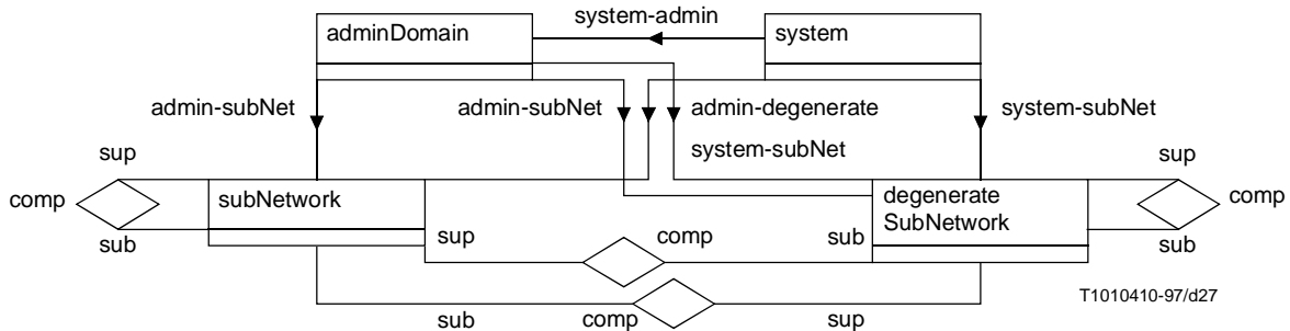
Figure I.2/Z.360 – Example GDMO specification after completion of the inheritance stage
