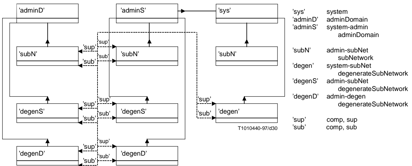
Figure I.5/Z.360 – Example classes for instantiation
