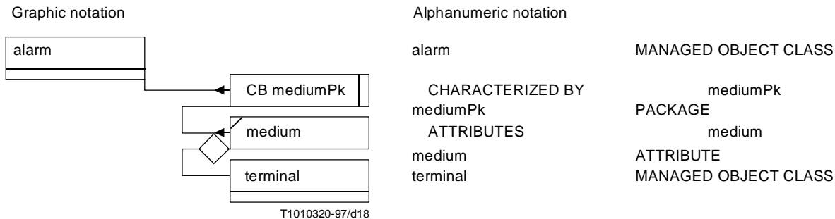
Figure 18/Z.360 – One-way reference
