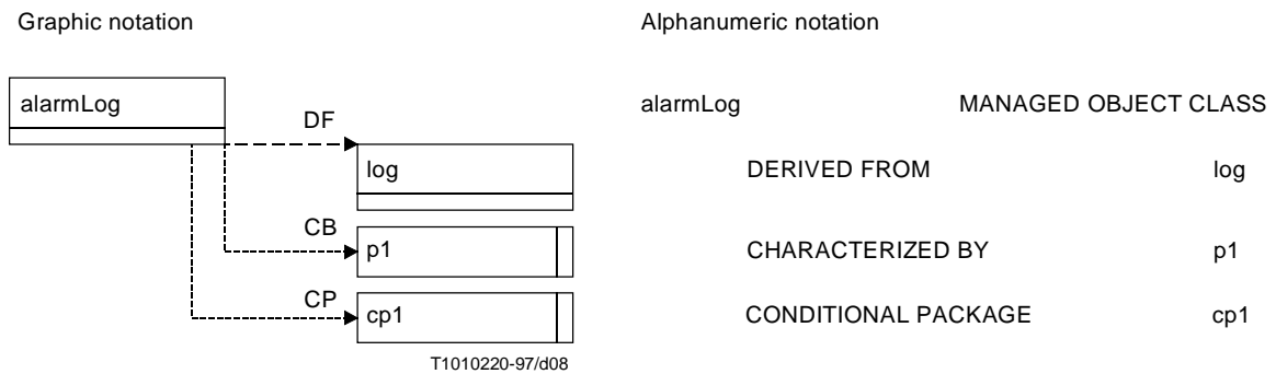
Figure 8/Z.360 – Shorthand notation
