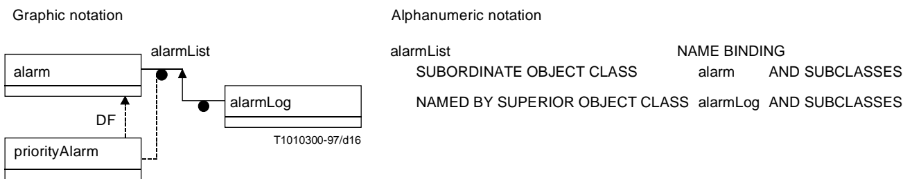
Figure 16/Z.360 – Indication of subclasses for which the Name Binding applies
