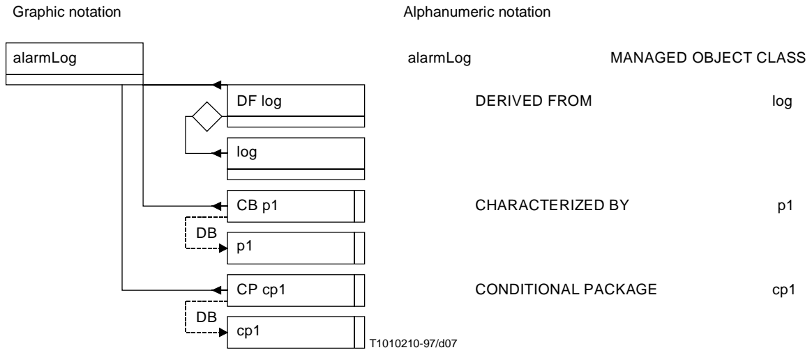
Figure 7/Z.360 – Managed Object Class template
