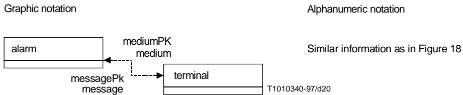
Figure 20/Z.360 – Two-way reference
