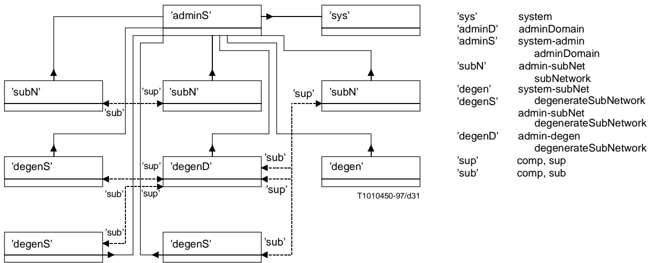
Figure I.6/Z.360 – Example instances
