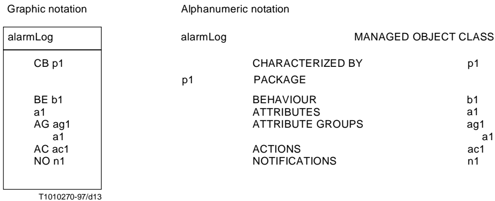
Figure 13/Z.360 – Combined notation
