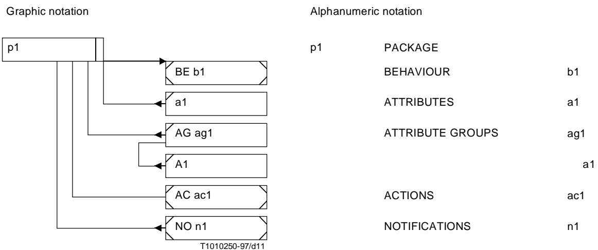
Figure 11/Z.360 – Package template
