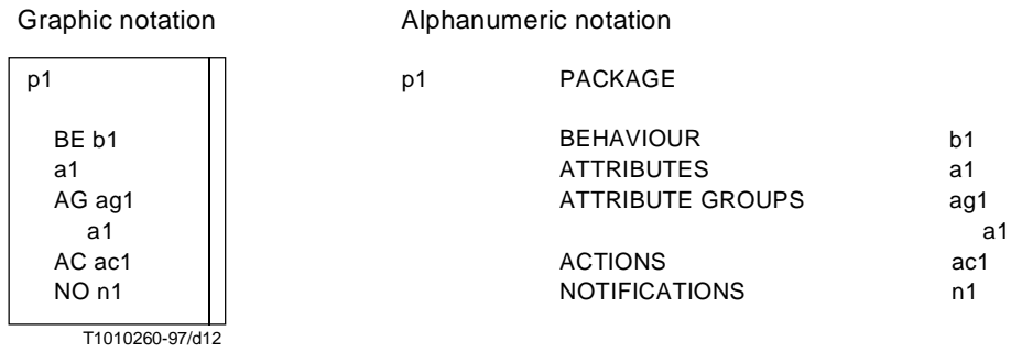
Figure 12/Z.360 – Compact notation
