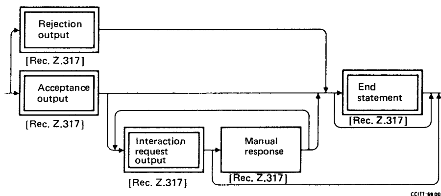
FIGURE 5/Z.323 Input acknowledgement
