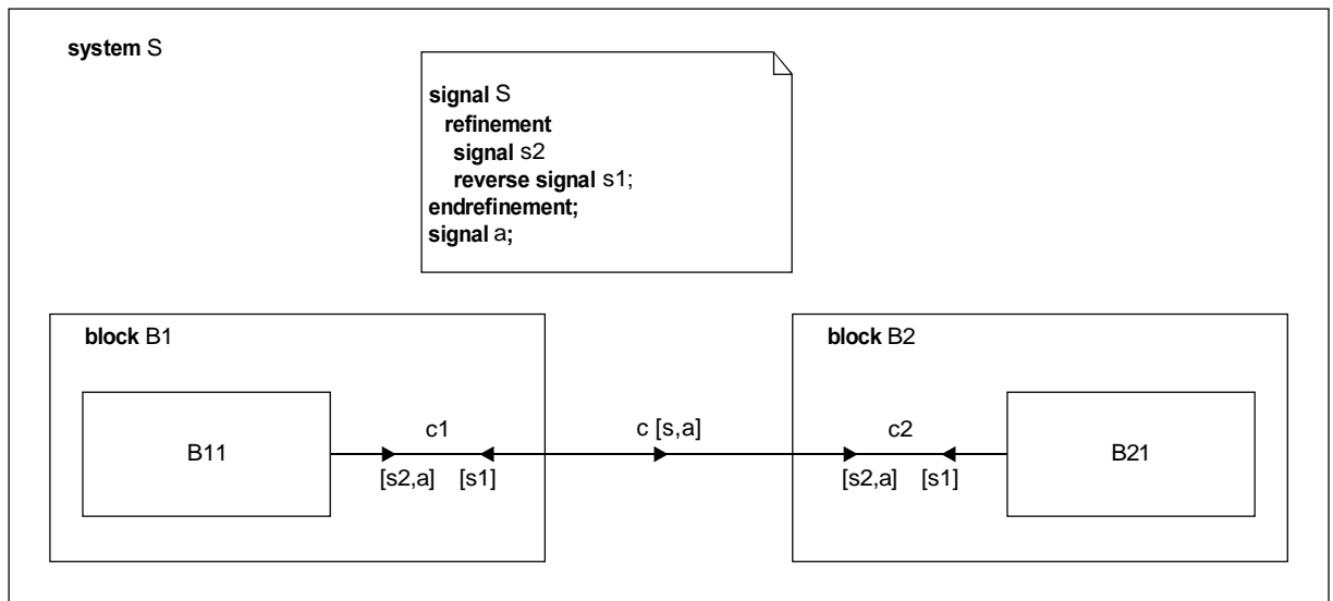
FIGURE 3.3.1/Z.100 System diagram containing signal refinement
