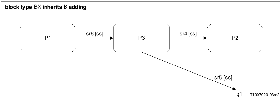
FIGURE 6.4.6/Z.100 Definition of subtype (SDL/GR)
