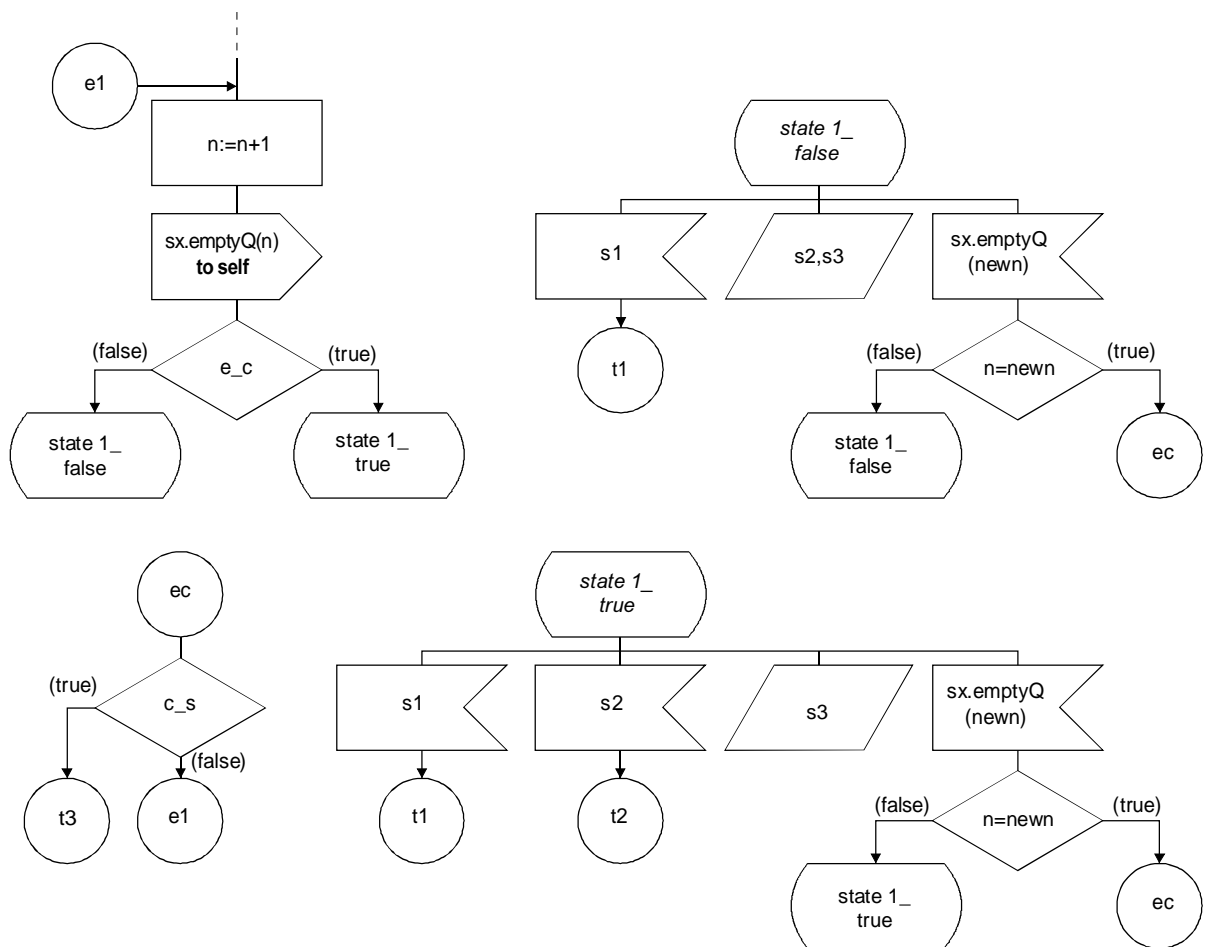
FIGURE 4.12.1/Z.100
