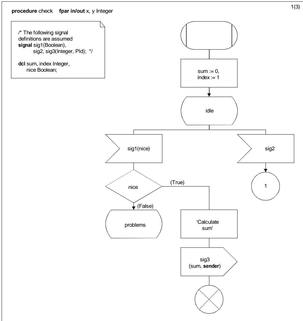
FIGURE 2.10.12/Z.100
