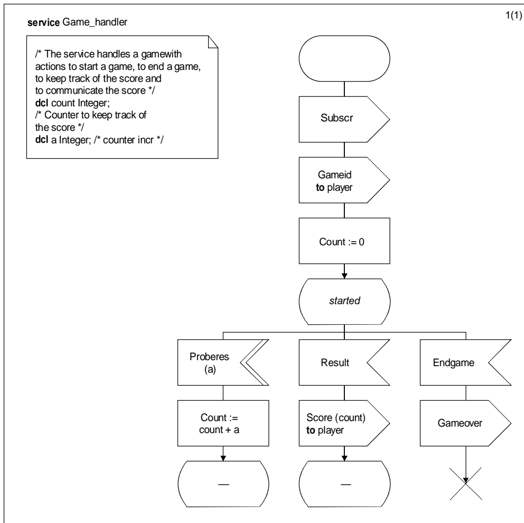
FIGURE 2.10.18/Z.100
