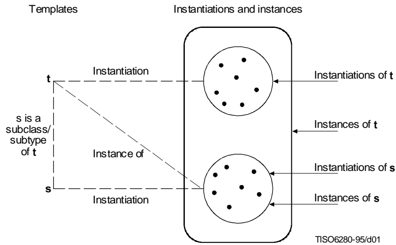
Figure 1 – Relationship between templates, instantiations and instances
