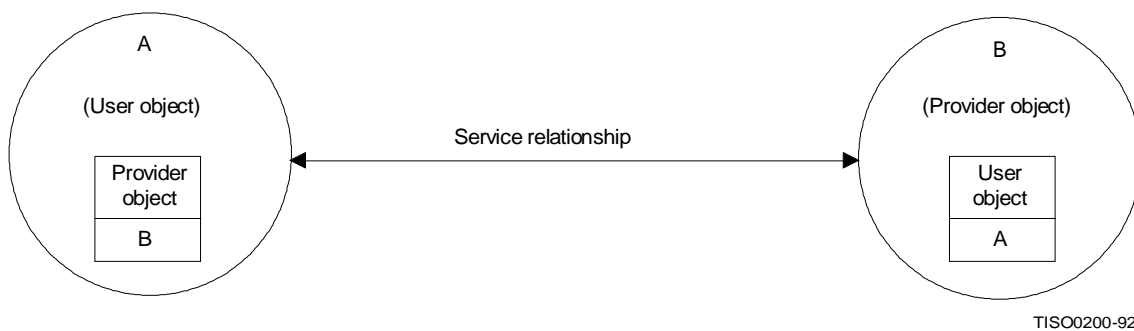
Figure 2 – Relationship roles
