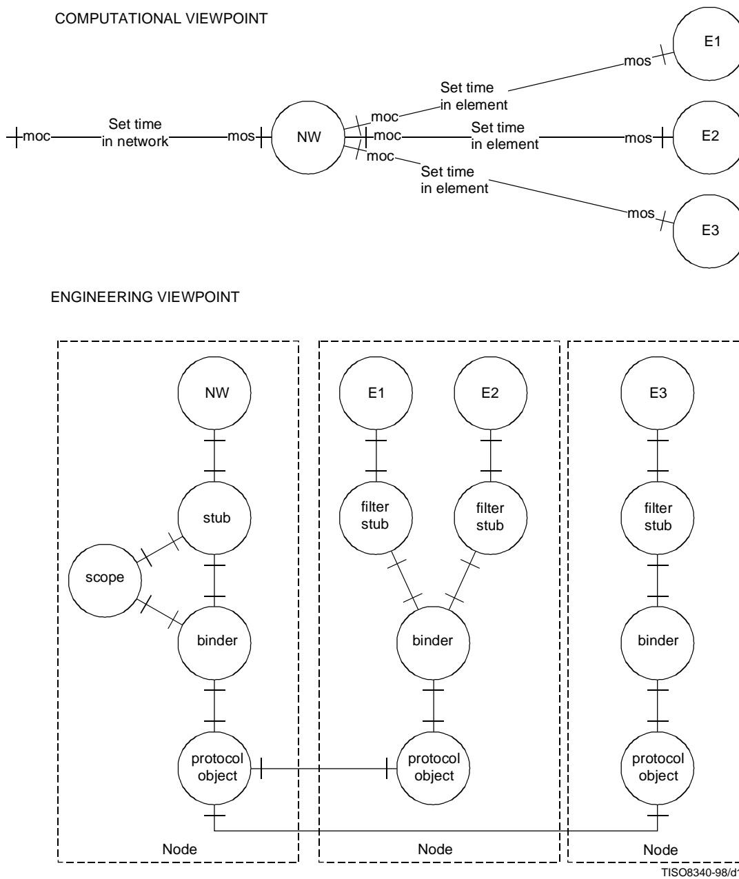
Figure 12 – Scoping and filtering as an engineering optimisation (not exposed computationally)
