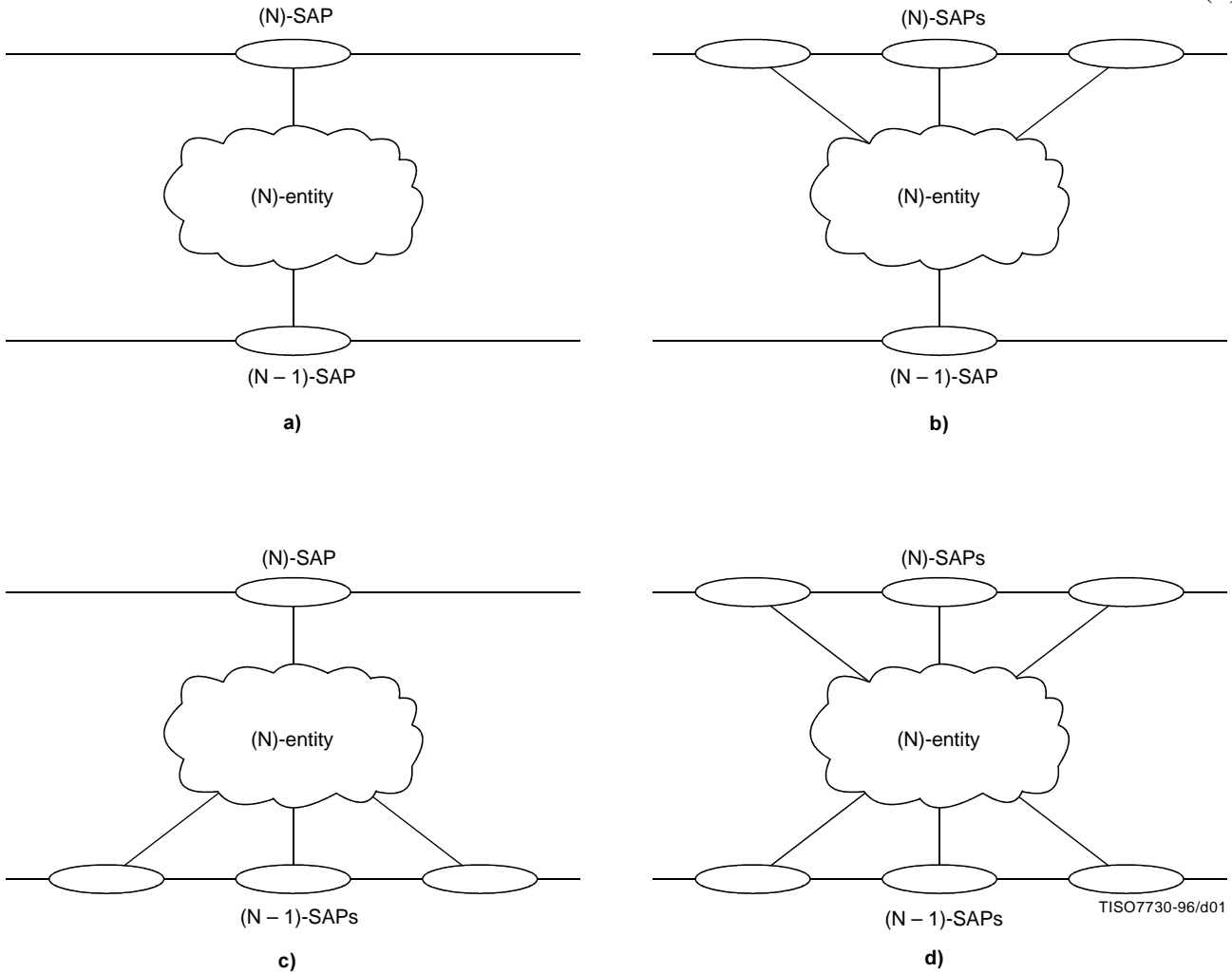
Figure 1 – Relationships of (N)-entity to (N)-SAPs and to (N – 1)-SAPs
