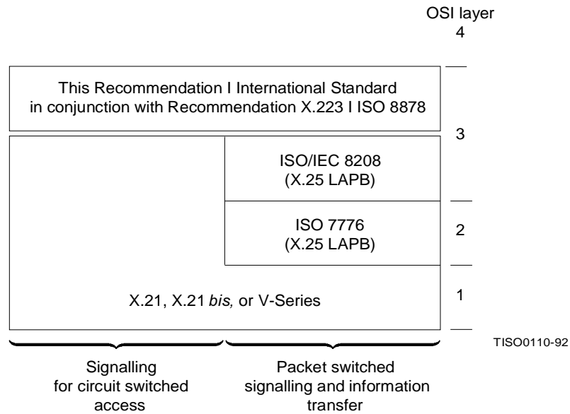
Figure 4 – Protocol layers at R reference point
