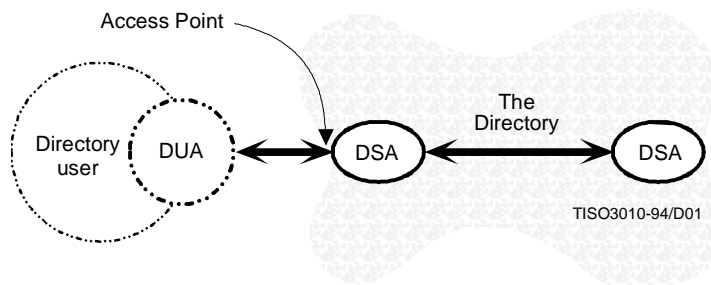
Figure 1 – Directory Interactions
