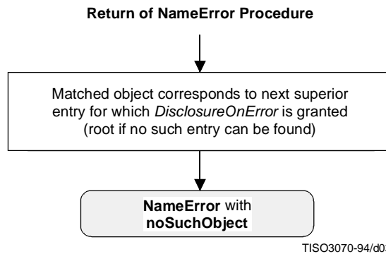
Figure B.2 – Return of Name Error
