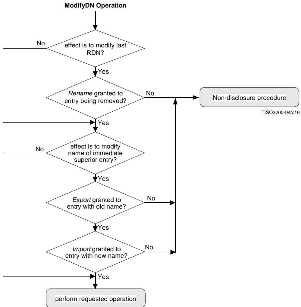
Figure B.15 – ModifyDN Operation
