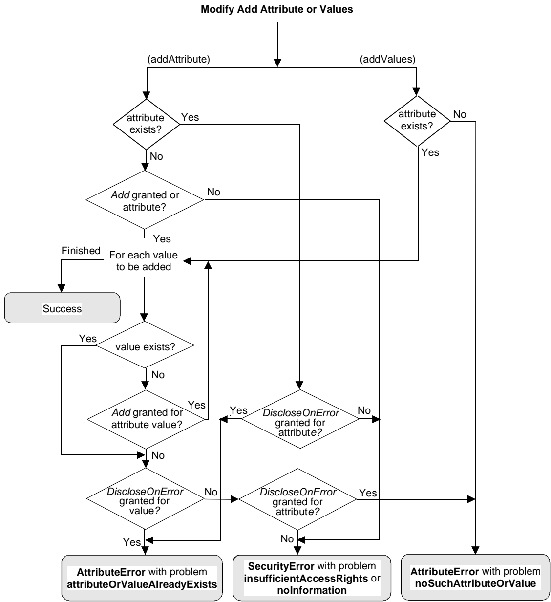
Figure B.16 – Modify Add Attribute or Values
