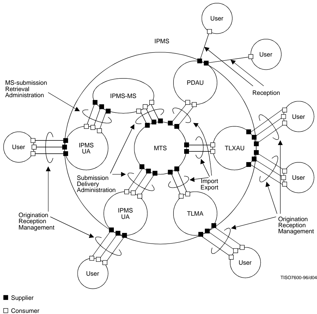
Figure 4 – The Interpersonal Messaging System
