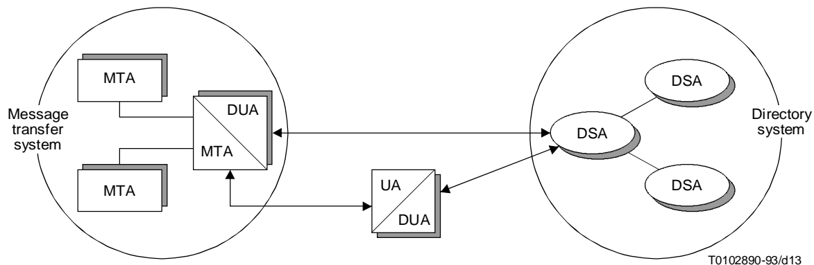
FIGURE 13/F.400 Functional model of MHS-directory interworking
