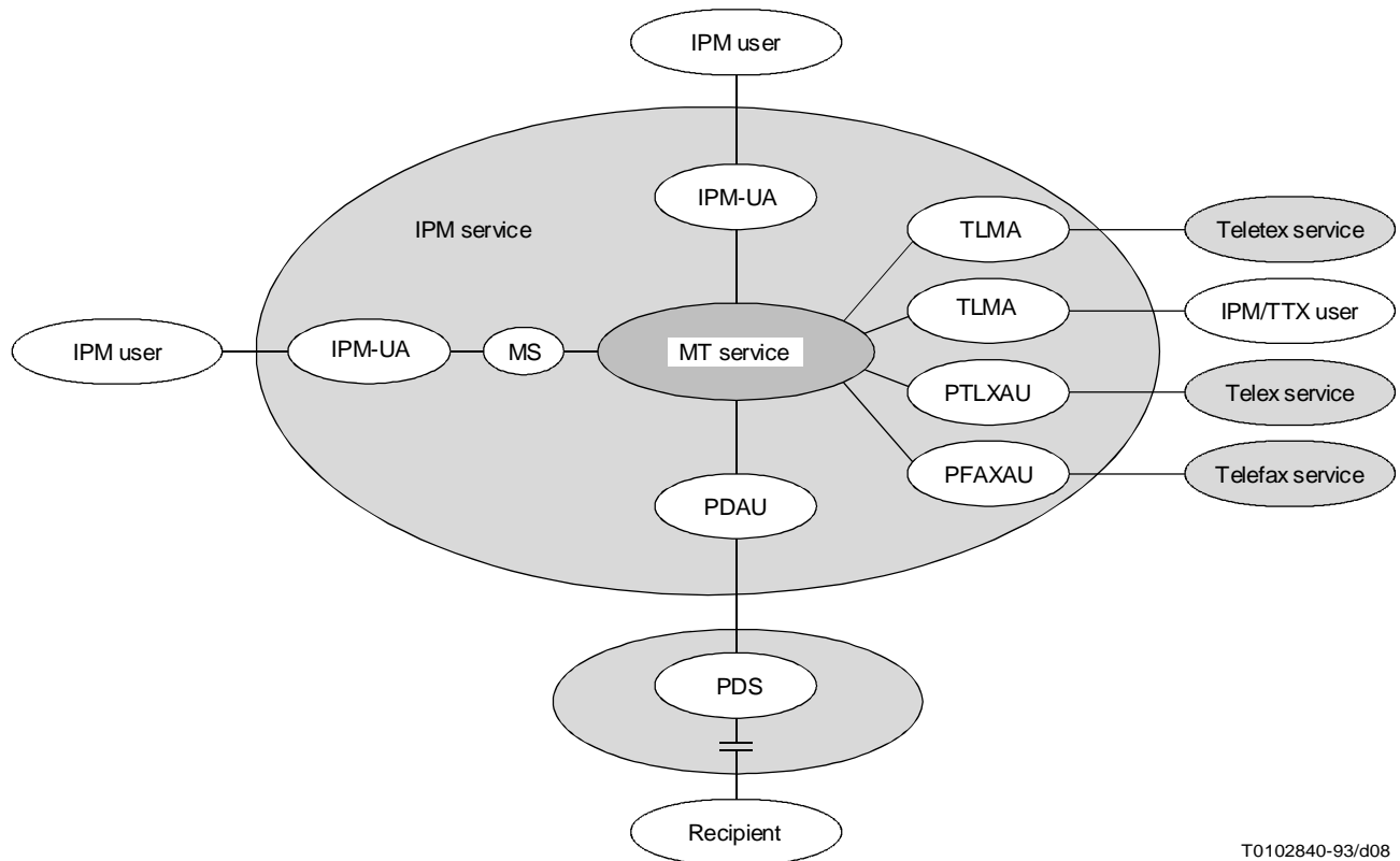
FIGURE 8/F.400 IPM service functional model
