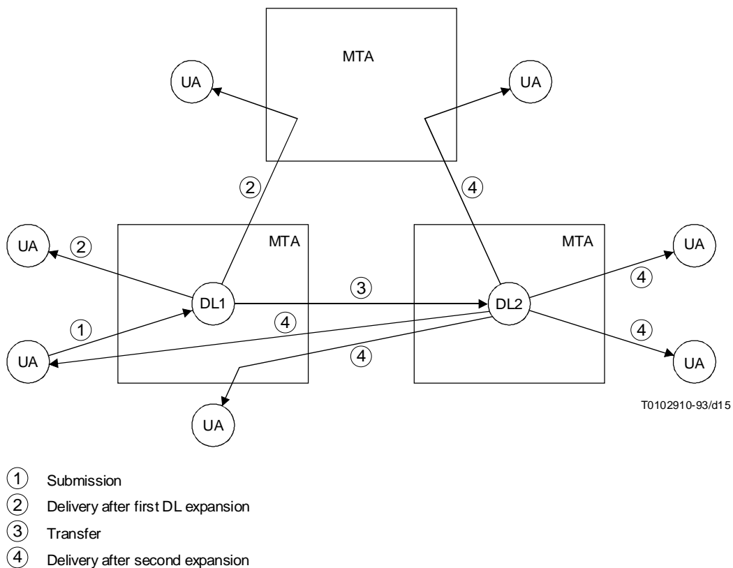
FIGURE 15/F.400 Distribution list expansion
