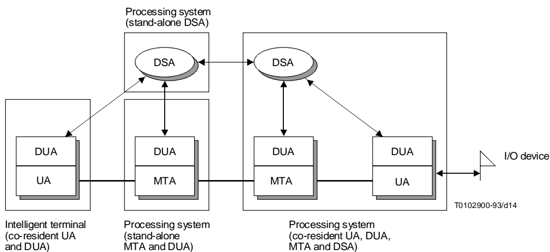
FIGURE 14/F.400 Physical configurations for MHS-directory interworking
