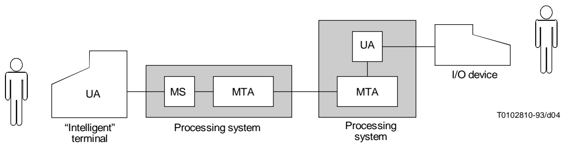
FIGURE 3/F.400 Co-resident UA and MTA
