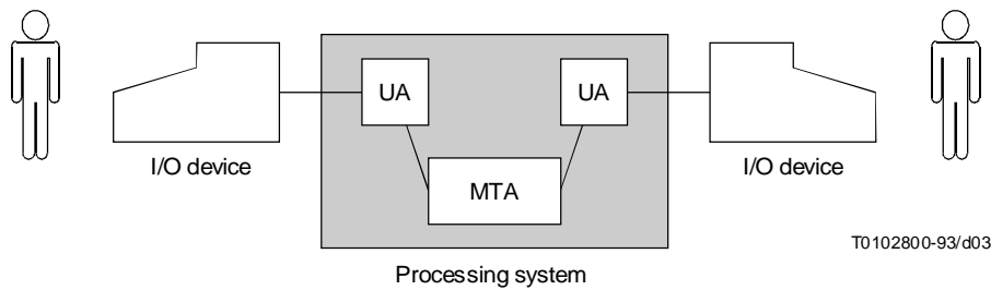
FIGURE 3/F.400 Co-resident UA and MTA
