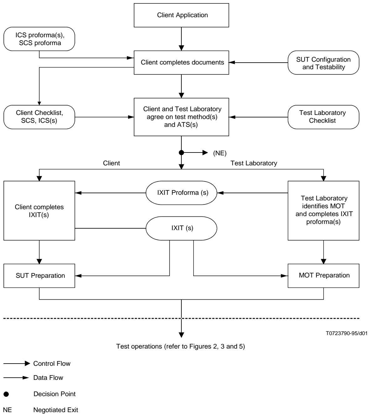
FIGURE 1/X.294 Preparation for Testing
