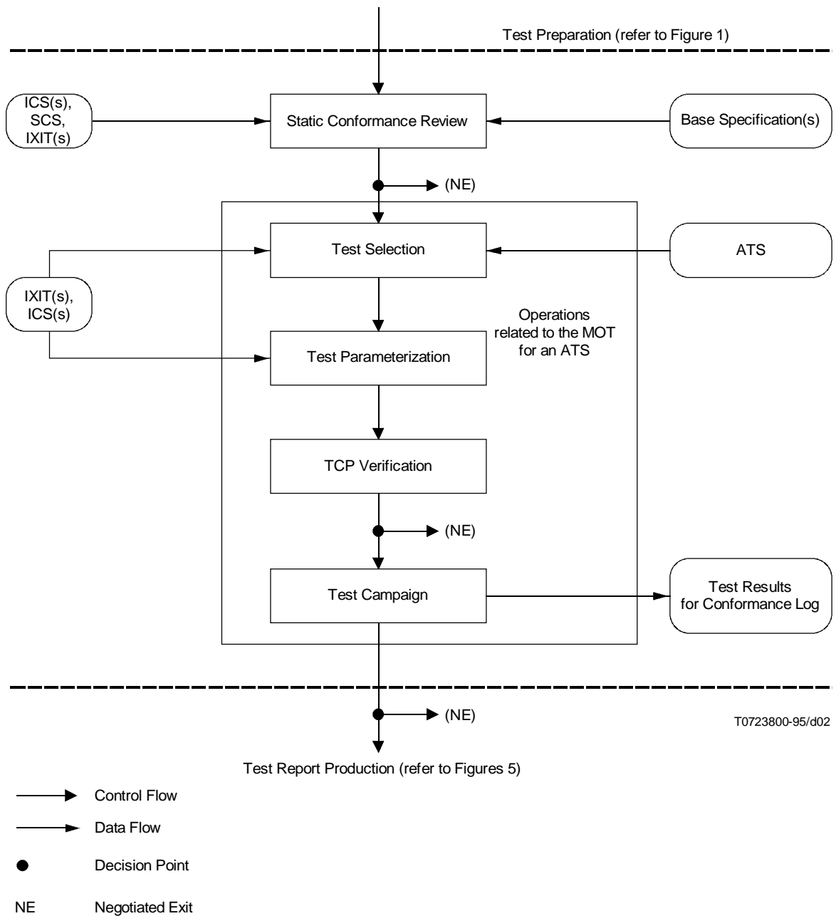
FIGURE 2/X.294 Typical Test Operations for a single ATS
