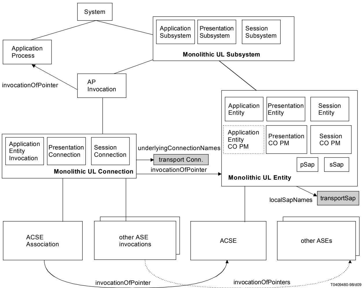
Figure A.1 – Monolithic Upper Layer Managed Object Classes and their Relationships
