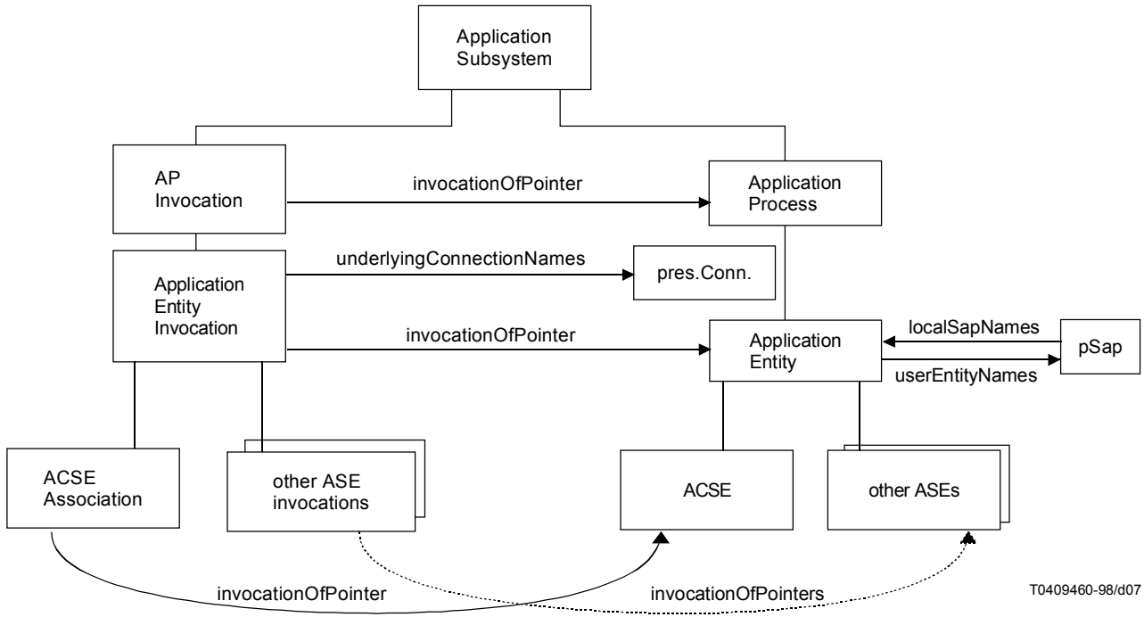
Figure 7 – Application Layer Containment Hierarchy with ACSE
