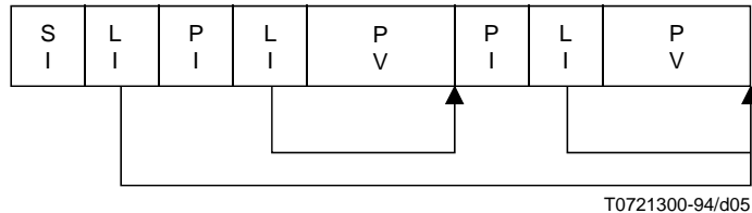
Figure 4 – Examples of SPDU structure
