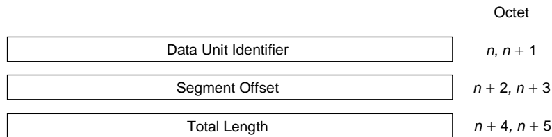
Figure 5 – PDU header – Segmentation part
