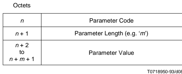
Figure 7 – Encoding of option parameters
