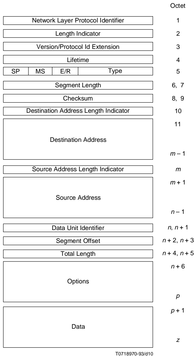
Figure 9 – Data PDU
