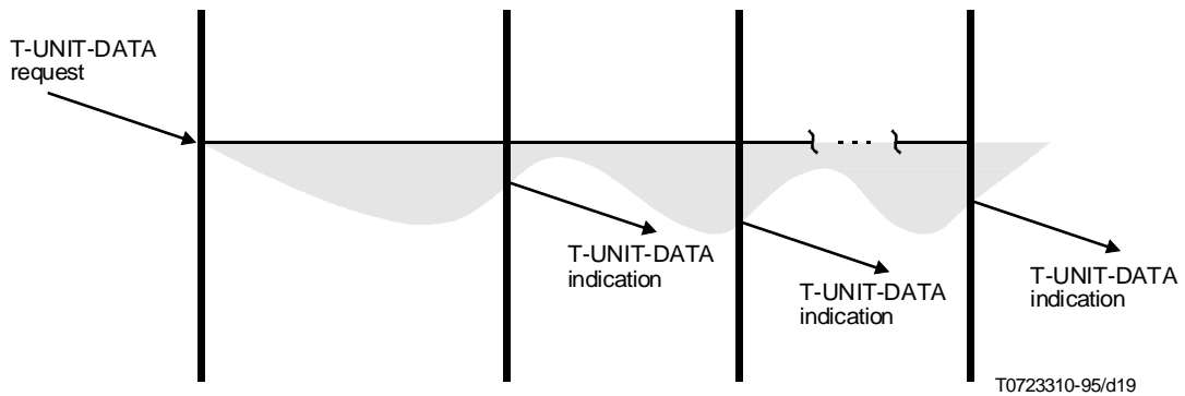
Figure 16b – Sequence of primitives in a successful multicast transport connectionless-mode transmission
