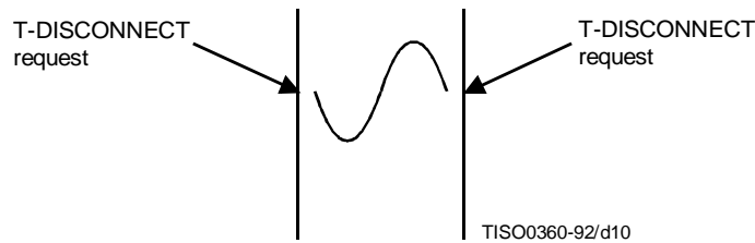
Figure 9 – Sequence of primitives in simultaneous TS users invoked release
