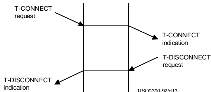
Figure 12 – Sequence of primitives in a TS user rejection of a TC establishment attempt
