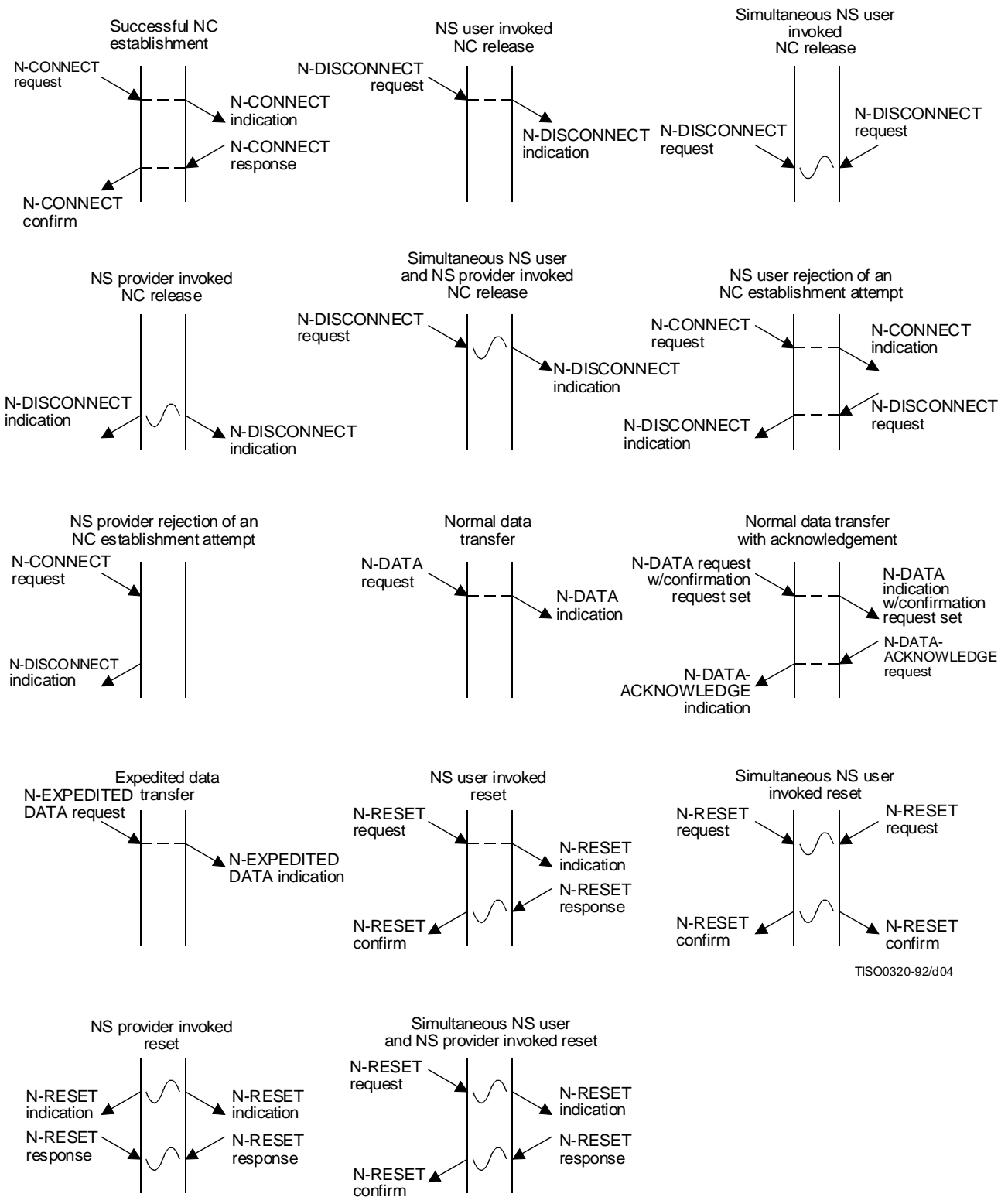
Figure 3 – Summary of Network Service primitive time sequence diagrams
