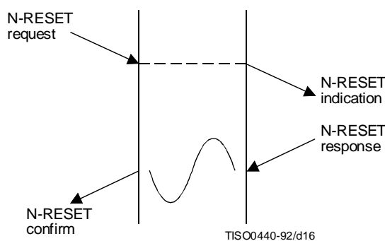
Figure 15 – Sequence of primitives in NS user invoked reset
