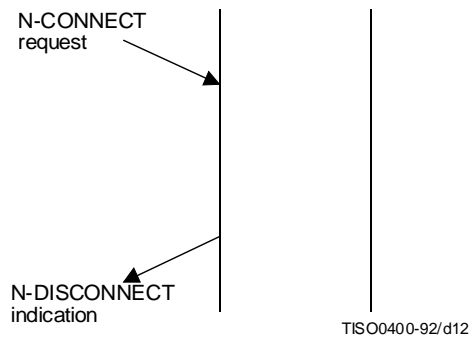
Figure 11 – Sequence of primitives in NS provider rejection of an NC establishment attempt
