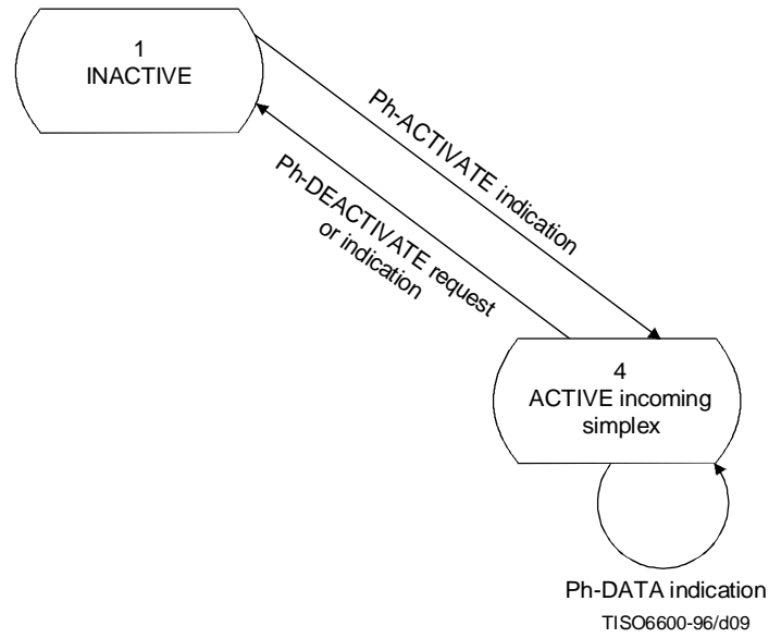
Figure 8 – State transition diagram for simplex mode, incoming
