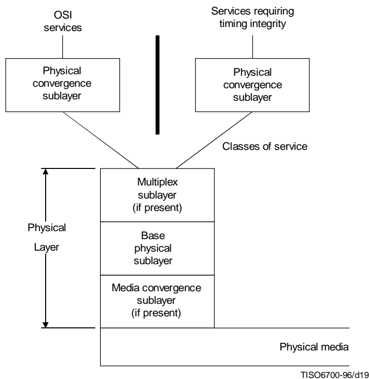
Figure A.1 – Structure of the Physical Layer
