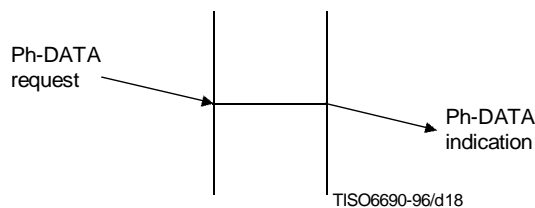
Figure 17 – Sequence of primitives in data transfer
