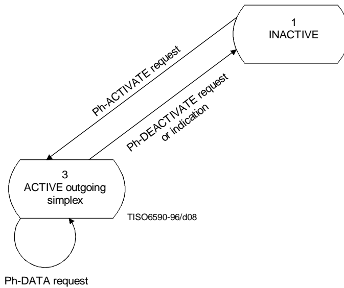
Figure 7 – State transition diagram for simplex mode, outgoing
