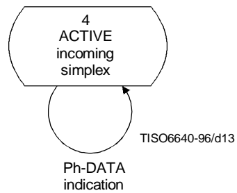
Figure 12 – State transition diagram for simplex mode, incoming, data transfer phase only
