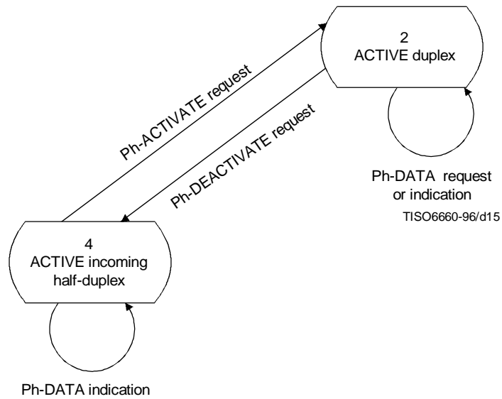
Figure 14 – State transition diagram for half-duplex/duplex mode shift
