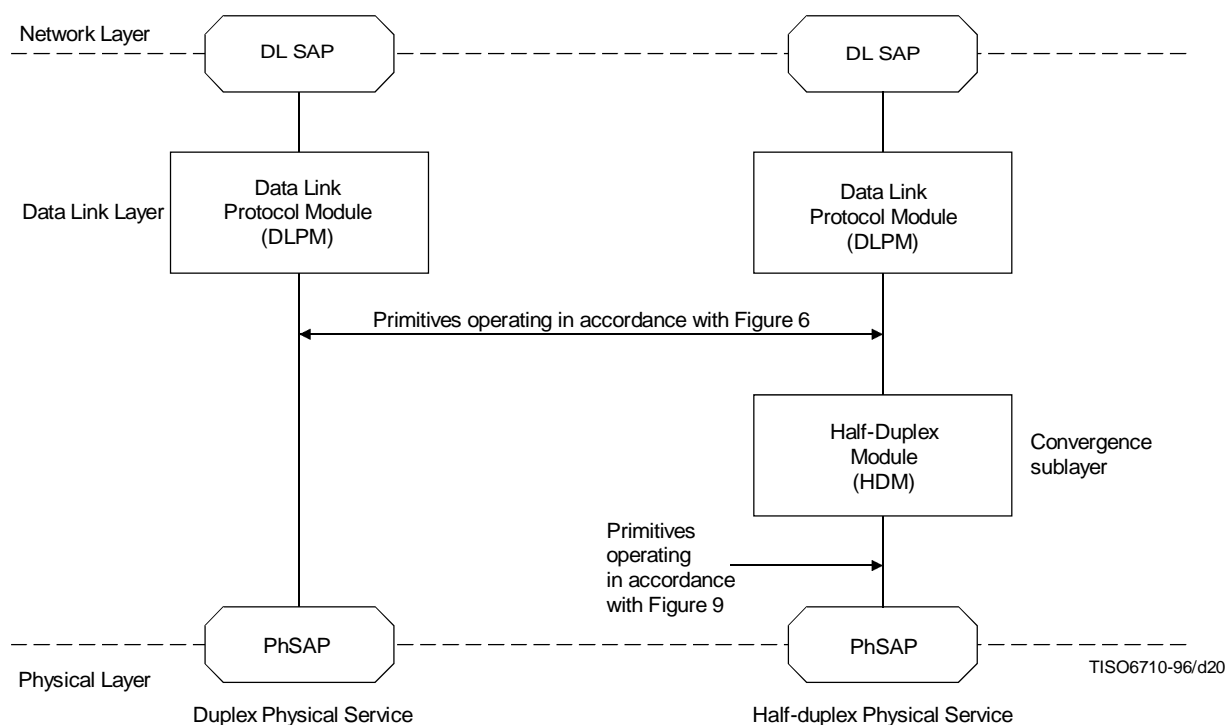
Figure B.1 – Structure of the data link layer
