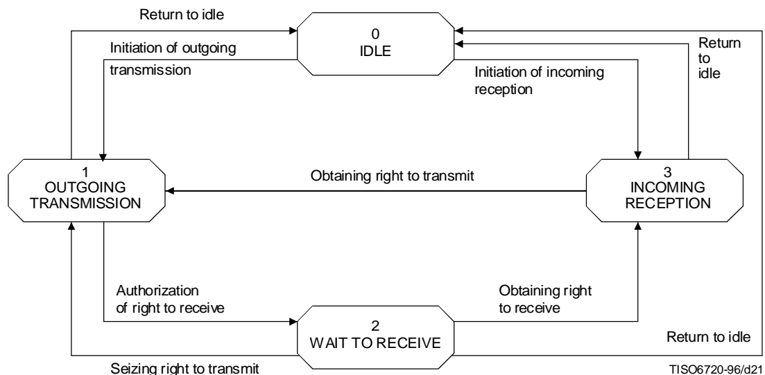
Figure B.2 – State diagram for HDM
