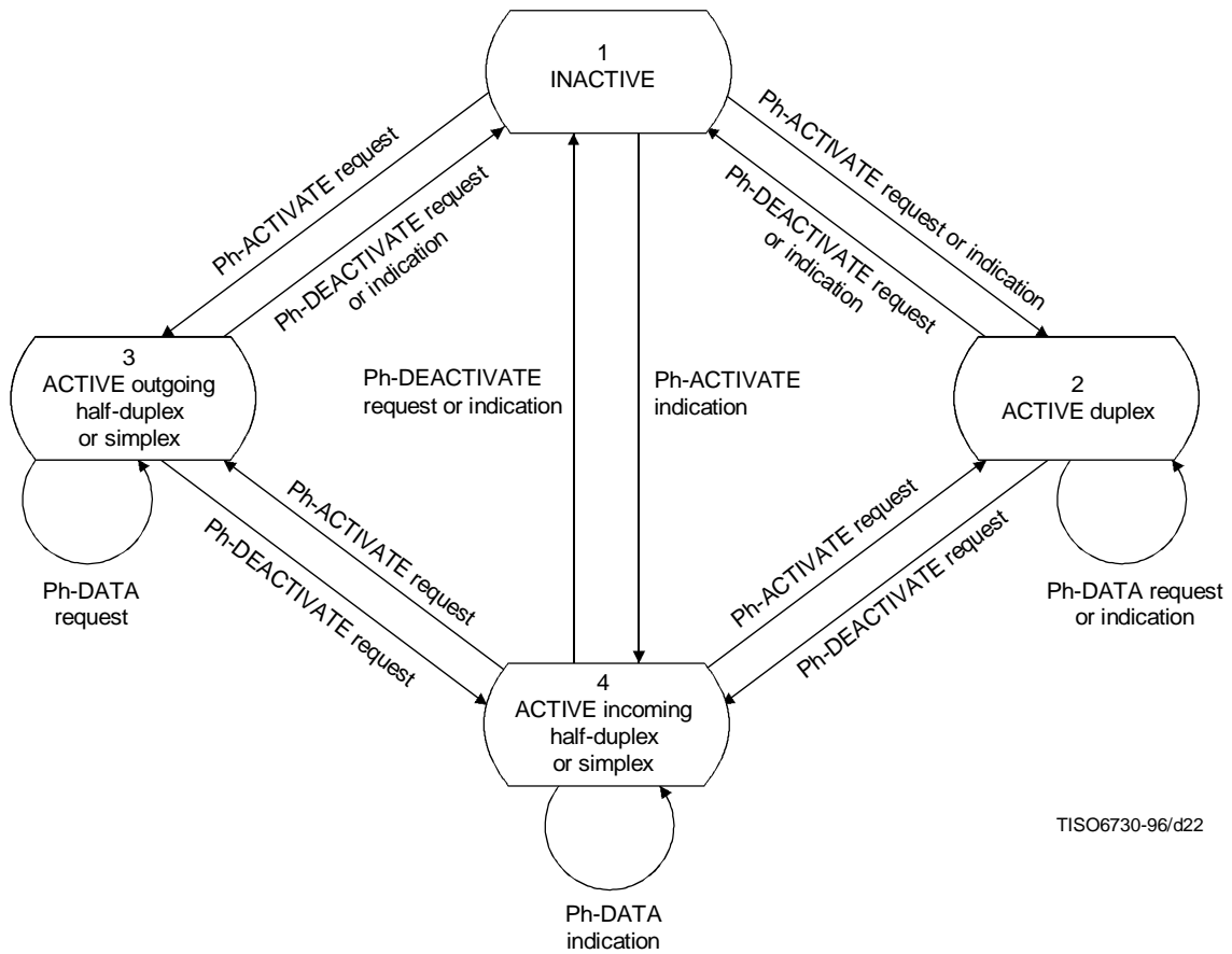
Figure C.1 – Composite state transition diagram for sequences of primitives at a PhC endpoint
