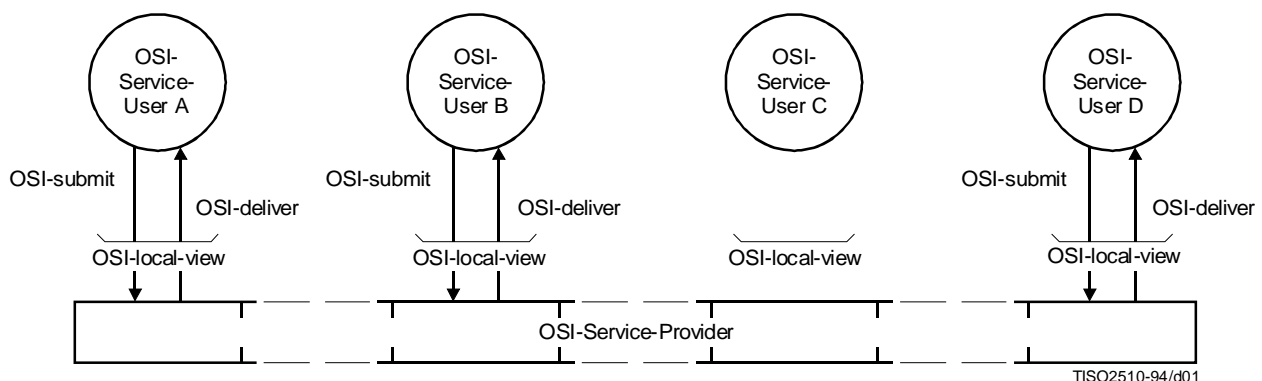
Figure 1 – OSI-service model
