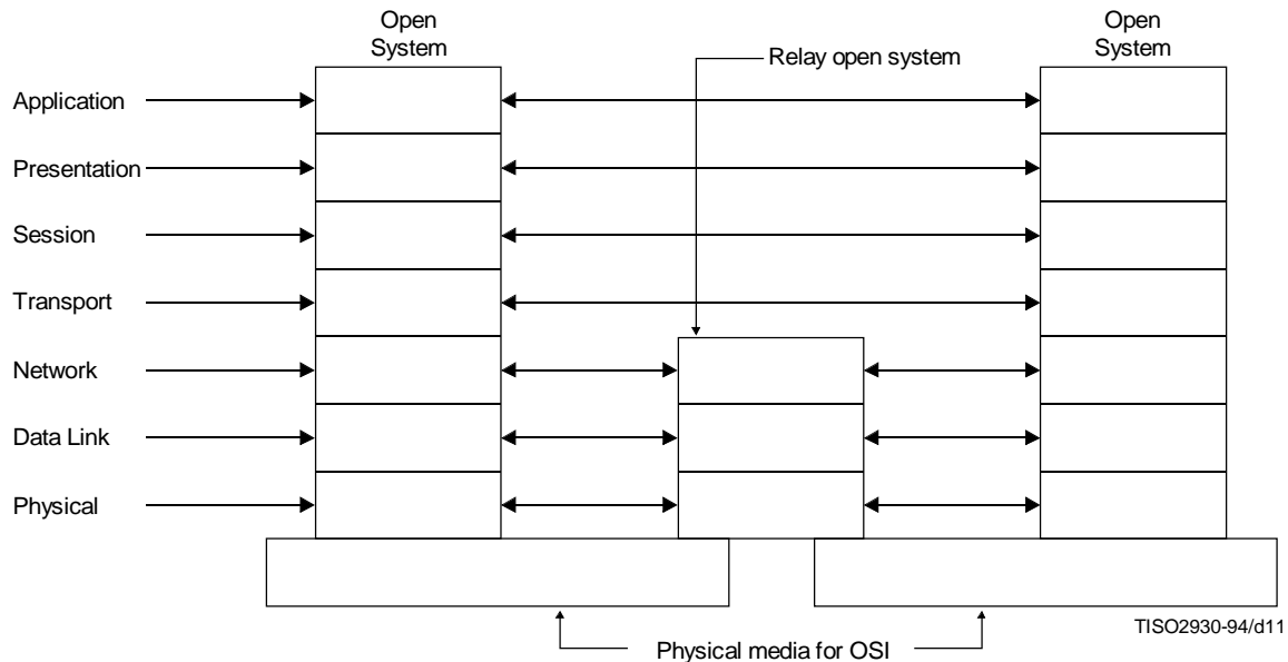
Figure 12 – Communication involving relay open systems
