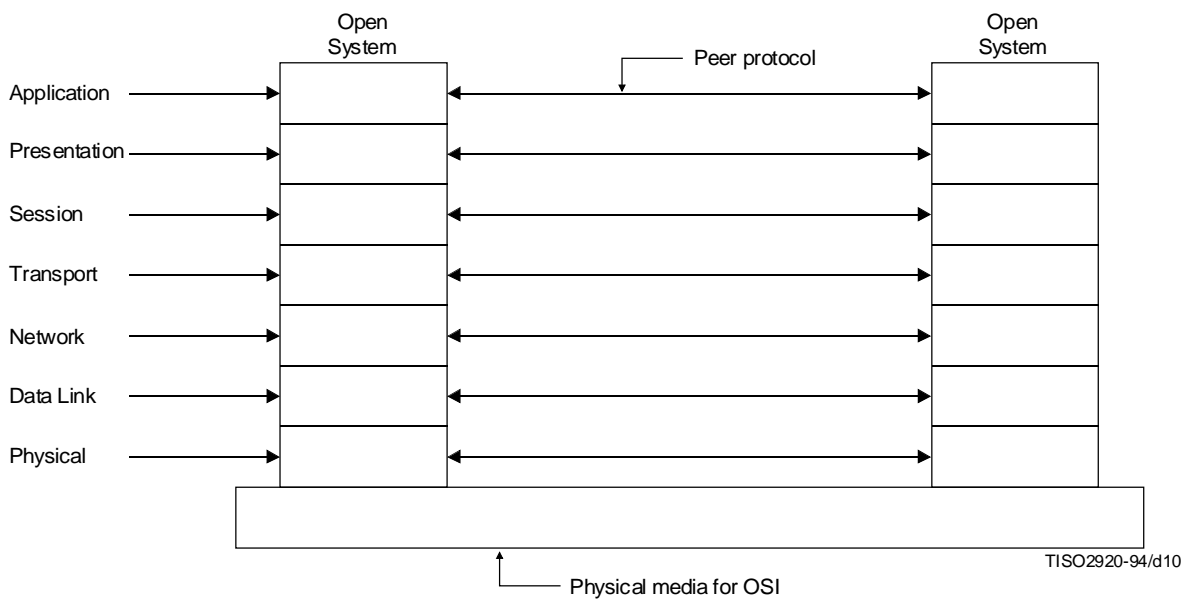
Figure 11 – Seven layer reference model and peer protocols
