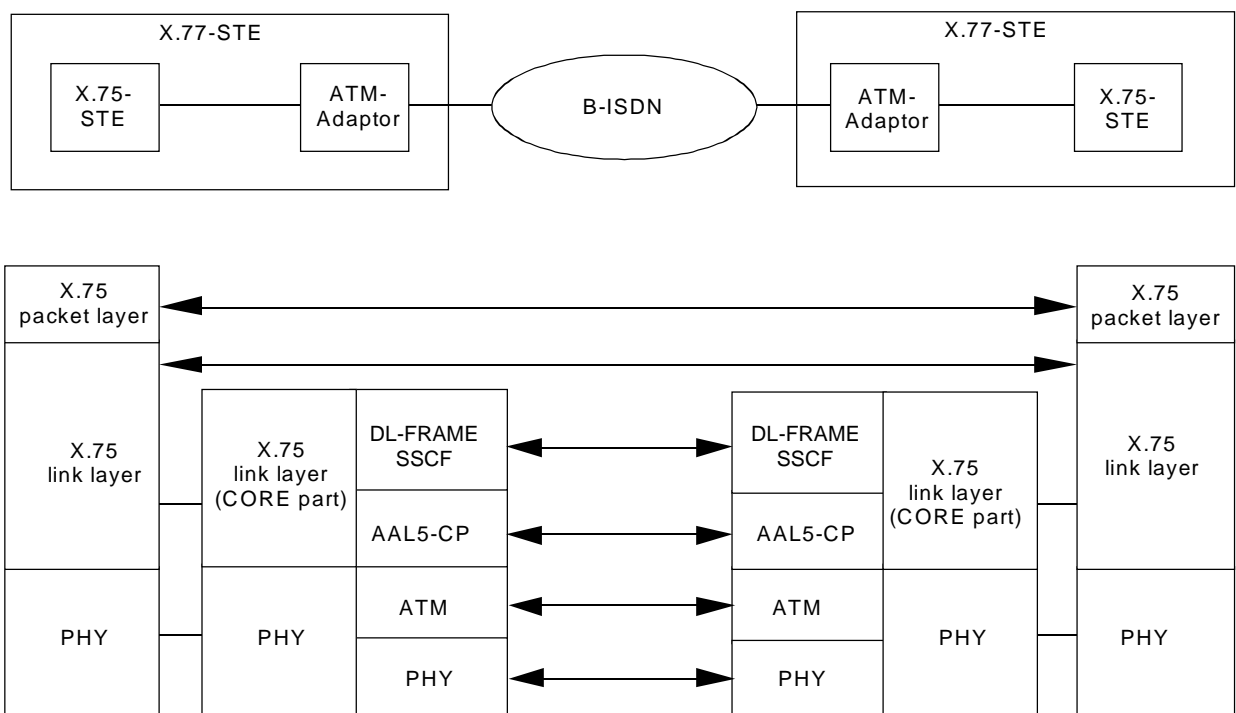
Figure 14-2/X.77 – Packet mode interworking using ATM-Adaptor
