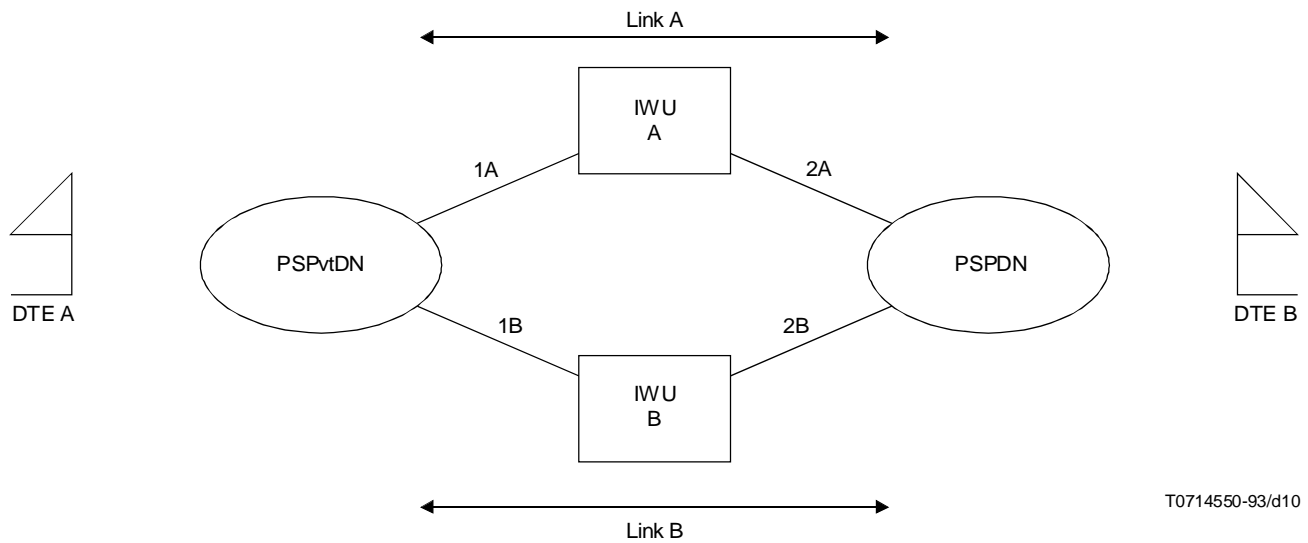
FIGURE 6/X.35 PSPDN/PSPvtDN alternate routing
