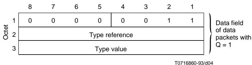
Figure 4/X.29 – Indication of break PAD message format
