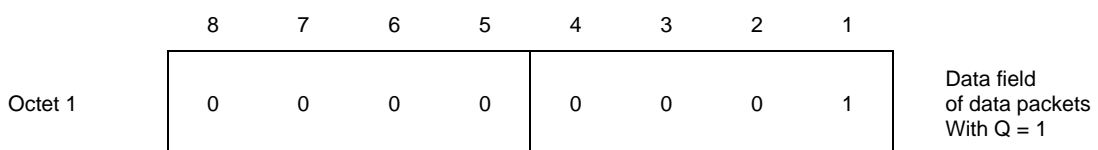
Figure 5/X.29 – Invitation to clear PAD message format
