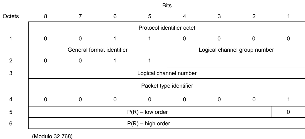
FIGURE 5-11/X.25 DTE and DCE RR packet format
