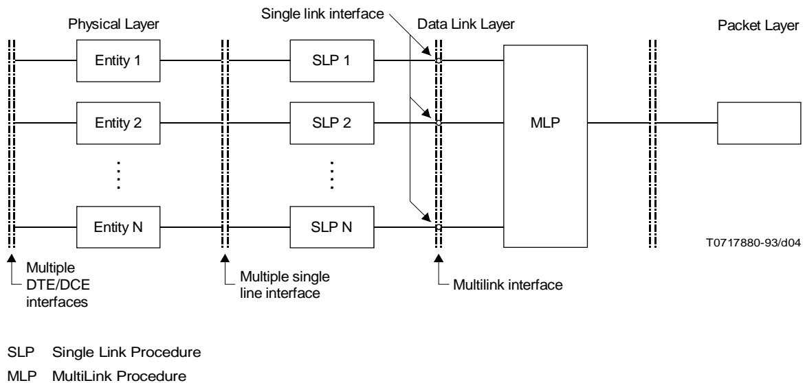
FIGURE 2-2/X.25 Multilink functional organization
