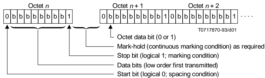
FIGURE 2-1/X.25
