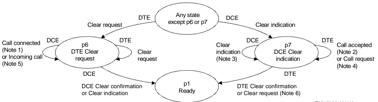
b) Call clearing phase
