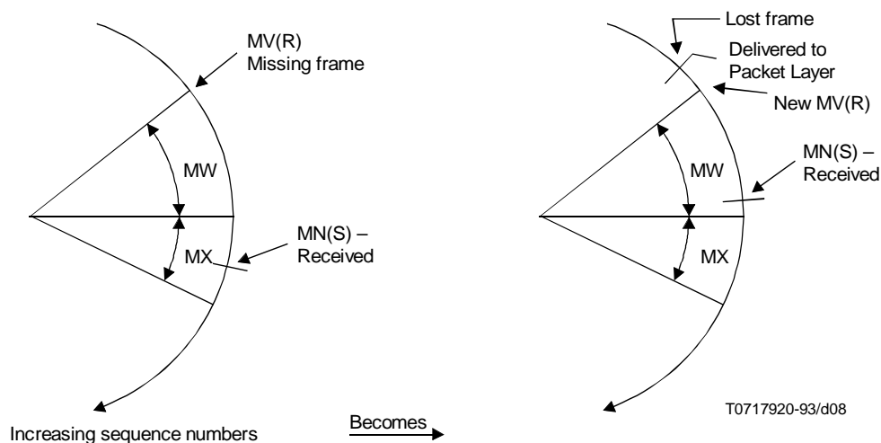
FIGURE 2-4/X.25 Detecting lost multilink frames
