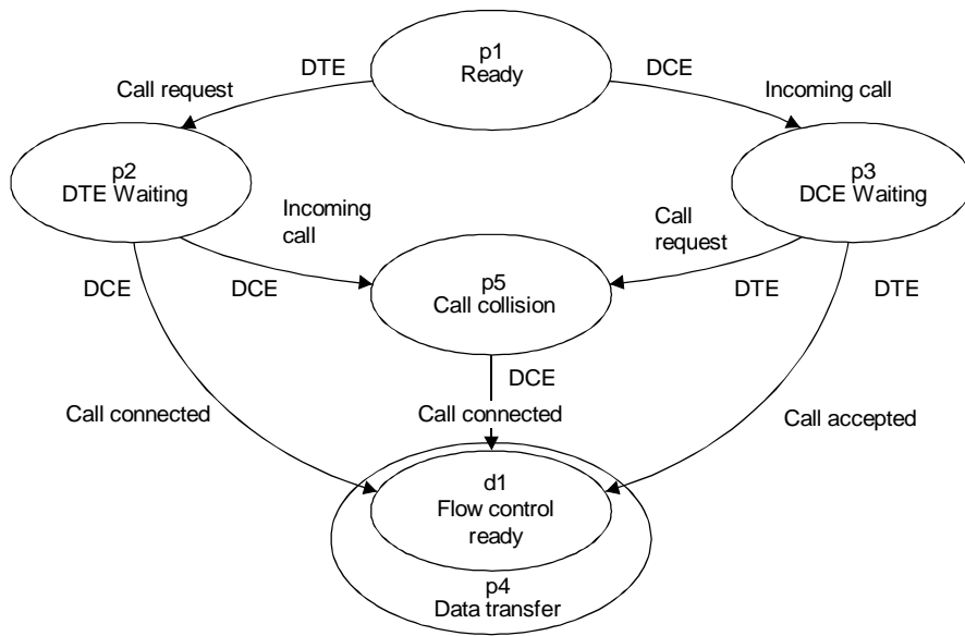
a) Call set-up phase
