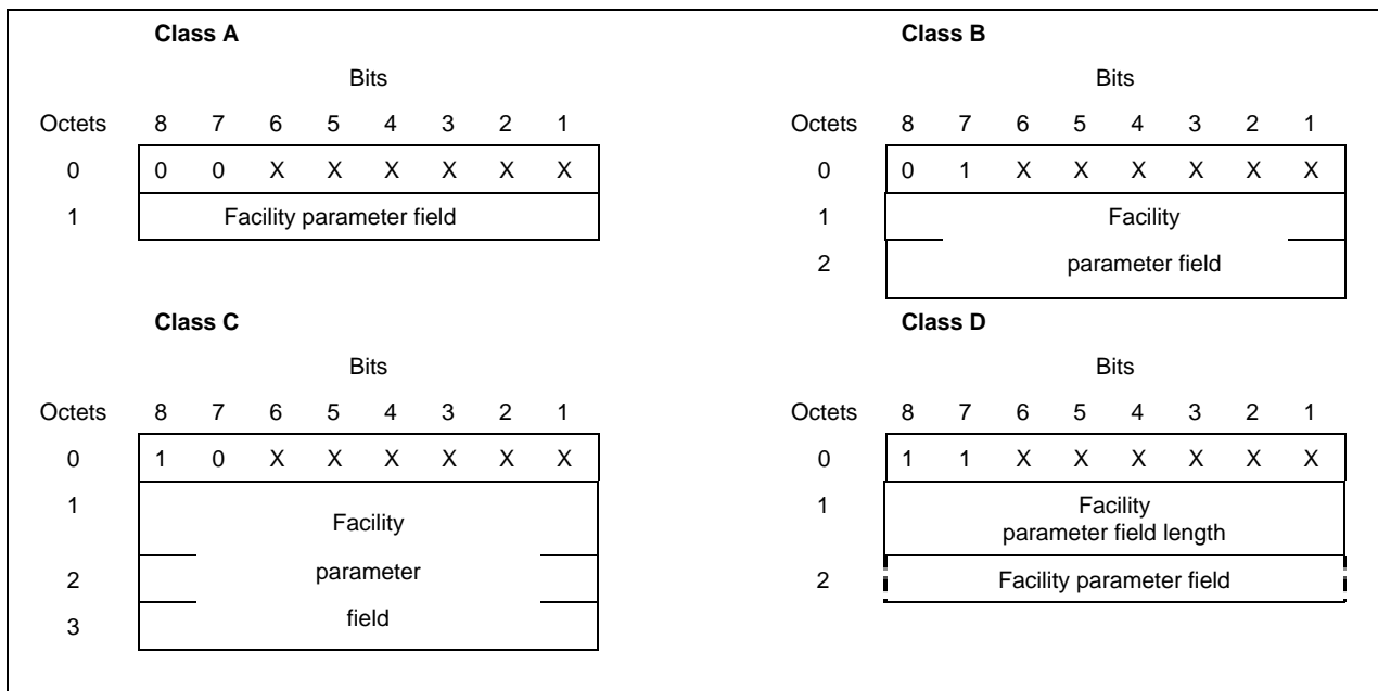
FIGURE 7-1/X.25
