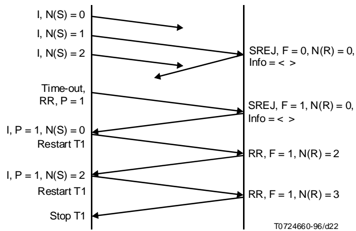
FIGURE VII.5/X.25
