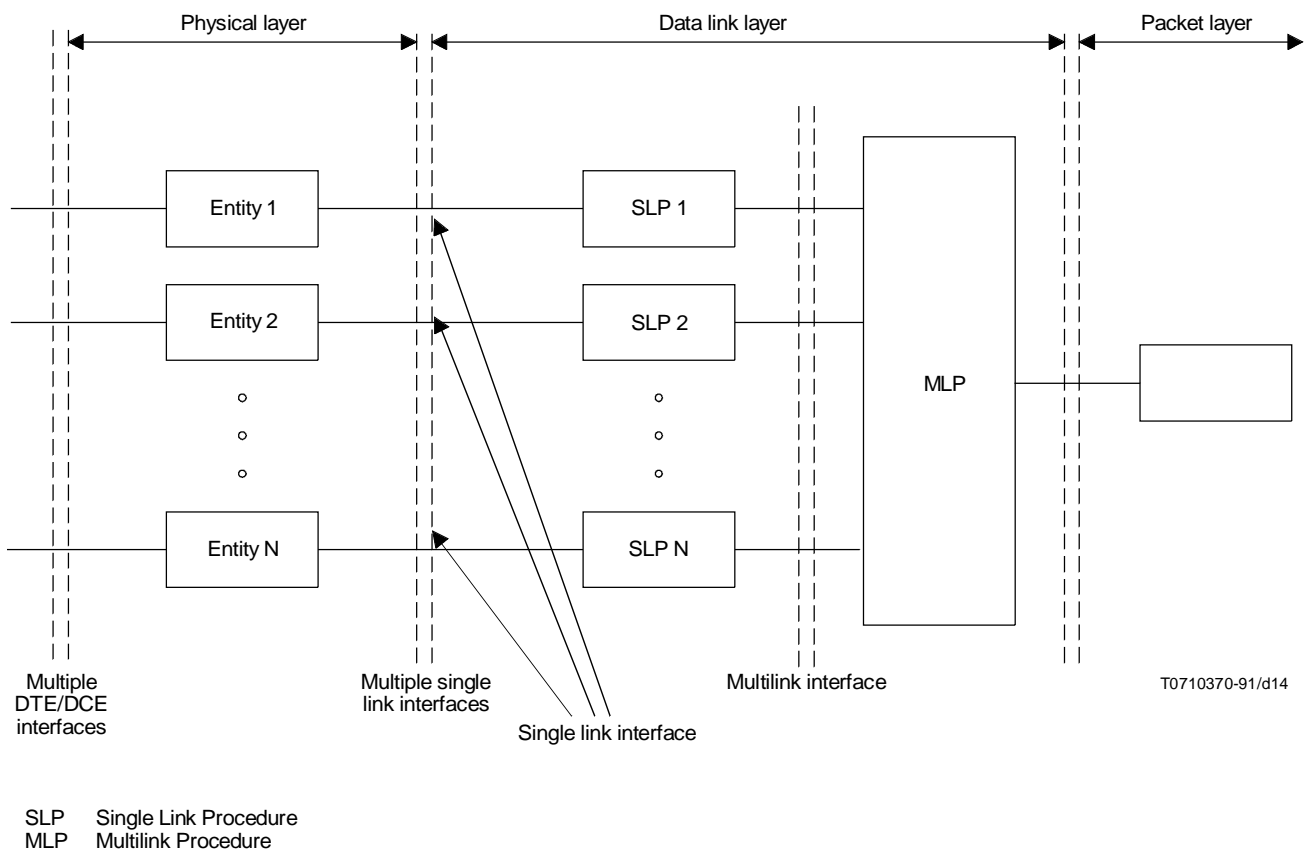
FIGURE 14/X.7 Multilink functional organization
