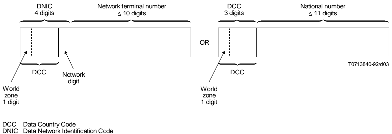
FIGURE 3/X.7 International data number X.121 format
