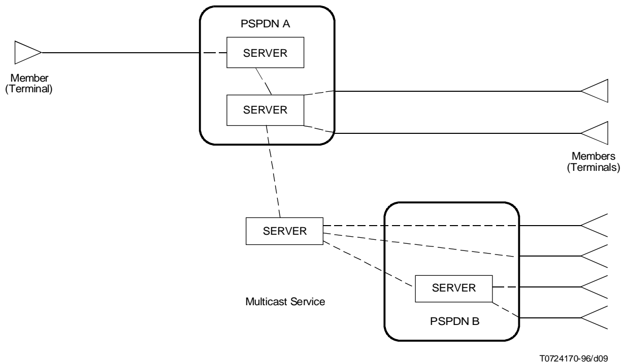
FIGURE 9/X.7 Example of multicast server implementation
