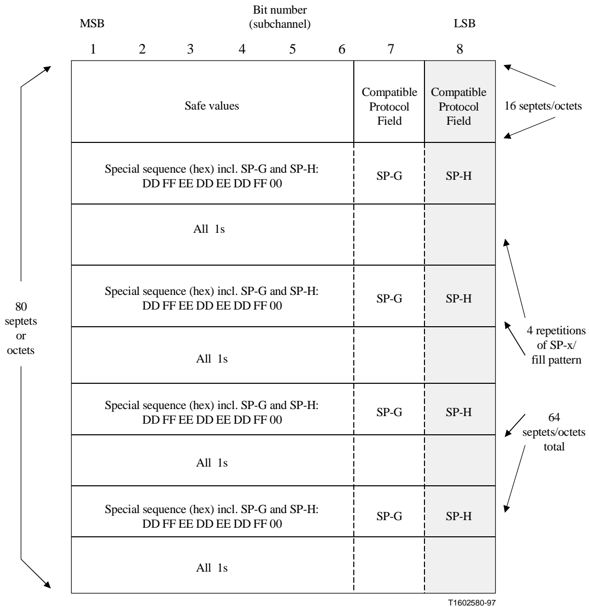
Figure 3/V.140 – Phase 1 signal for terminals attached to non-aligned channels (shaded bit position not present on 56C interfaces)
