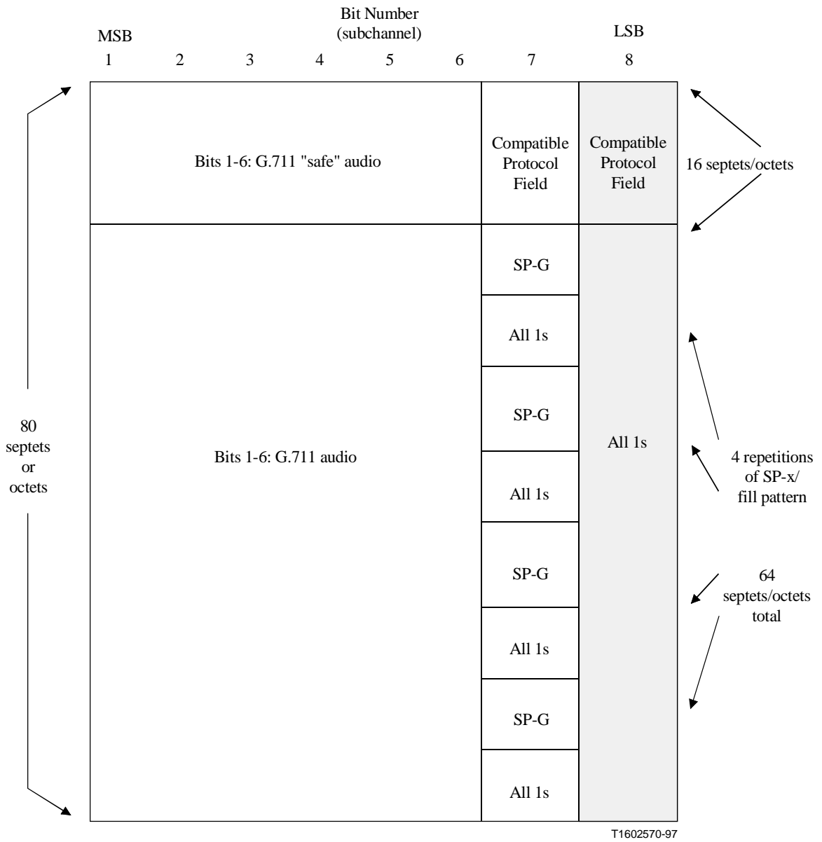
Figure 2/V.140 – Phase 1 signal for terminals attached to aligned channels (shaded bit position not present on 56C interfaces)
