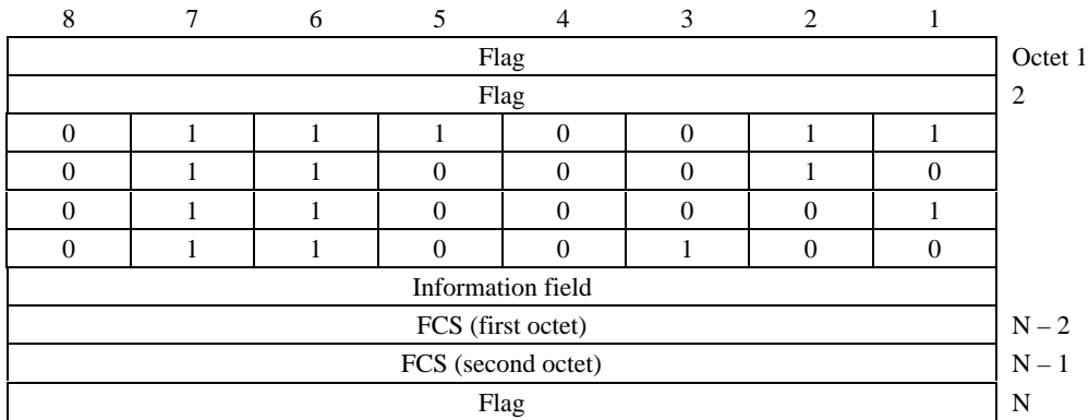
Figure 9/V.140 – Phase 3 message structure
