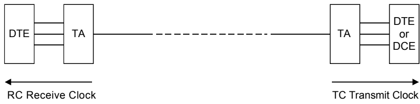
Case 1 – Receive clock tracks transmit clock via data or system synchronization.
