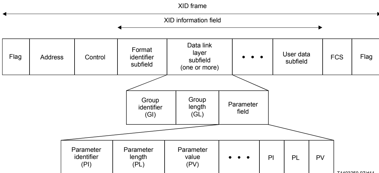
FIGURE C.1/V.120 General format of XID information field
