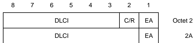
FIGURE 8/V.42 Address field format
